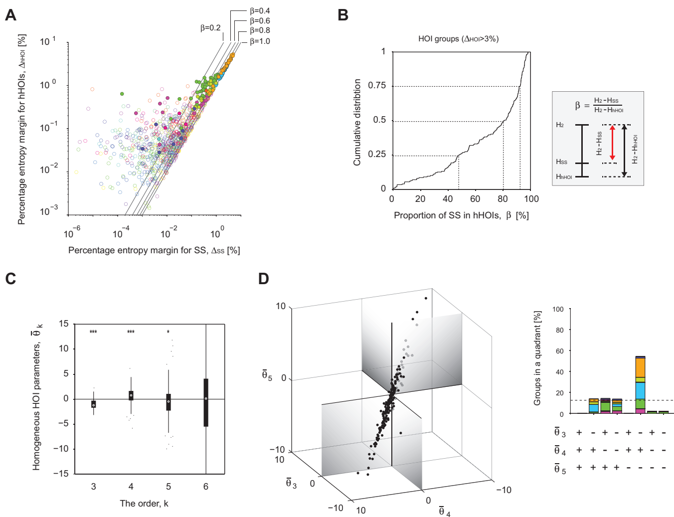
Figure 4 | The groups that express HOIs exhibited alternating signs of homogenous HOIs at successive orders of interaction. (A) Scatter plots of entropy margins for hHOIs versus entropy margins for SS. The same color indicates groups selected from the same slice culture. Filled circles indicate groups exhibiting HOIs ( \Delta_{\text{HOI}} > 3\% ). Dashed lines represent different proportions of homogenous HOI entropy margin explained by the SS term, \beta = \frac{H_2 - H_{\text{SS}}}{H_2 - H_{\text{hHOI}}} .
