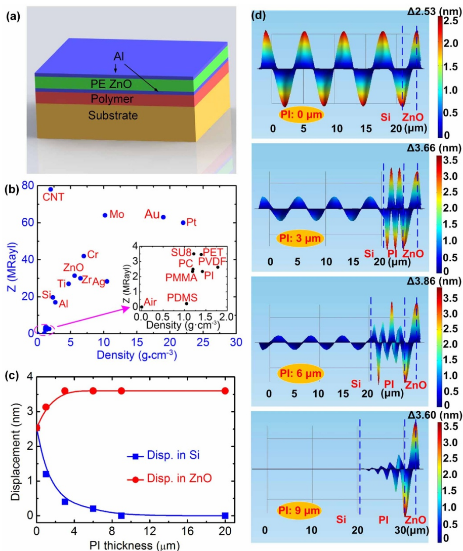
Figure 1 | Analysis and modeling of the FBAR with a polymer support layer architecture. (a) Schematic of the PI-FBAR architecture, (b) Comparison of acoustic impedance of various materials used in FBAR fabrication, (c) Summary of the displacements in the PE layer and Si in the PI-FBAR architecture as a function of PI layer thickness, (d) Displacements in layers of the PI-FBAR architecture with varying PI thickness, clearly showing the wave is confined and diminishes within the PI layer when its thickness is greater than 9 \mu\text{m} , and no acoustic energy is transmitted to the elastic Si substrate. The thicknesses of the ZnO and Si layers are 2.0 and 20 \mu\text{m} , respectively for the modeling. (Note Figure 1d is not based on an exact 2D figure, but rather viewed from a wide angle towards to narrow one. For clearer view, please see the 3D figures in Figure S2b in SI).
