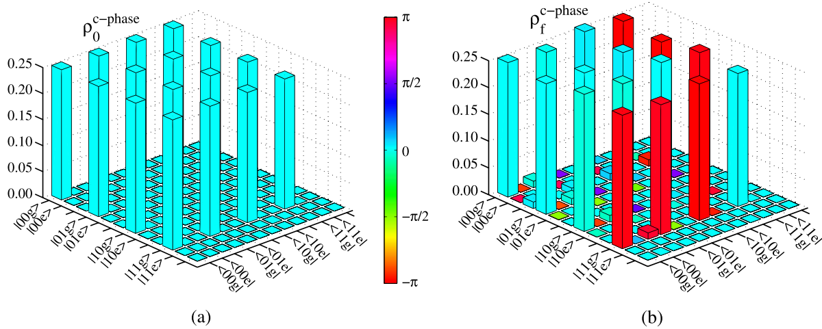
Figure 3 | (a) The density operator \rho_0 of the initial state |\psi_0\rangle of the quantum system composed of the two resonator qubits and the superconducting qutrit for constructing our c -phase gate. (b) The density operator \rho_f^{c\text{-phase}} . Here we take \theta_1 = \theta_2 = \frac{\pi}{4} .
