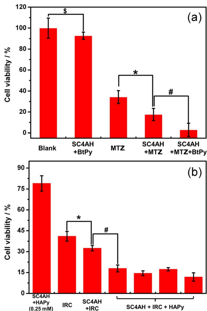
Figure 5 | (a) Cell viability of MCF7 cells after exposure to SC4AH–MTZ coassembly for 48 h at 37°C. [MTZ] = 0.01 mM, [SC4AH] : [MTZ] : [BtPy] = 2 : 3 : 2. ^{\$}P > 0.05 , ^{*}P < 0.01 and ^{\#}P < 0.05 . (b) Cell viability of MCF7 cells after exposure to SC4AH–IRC coassembly for 48 h at 37°C. [IRC] = 0.05 mM, [SC4AH] : [IRC] = 1 : 4. ^{*}P < 0.01 and ^{\#}P < 0.001 . In the SC4AH + IRC + HAPy entry, [HAPy] = 0.0125, 0.05, 0.1 and 0.25 mM, respectively (from left to right).
