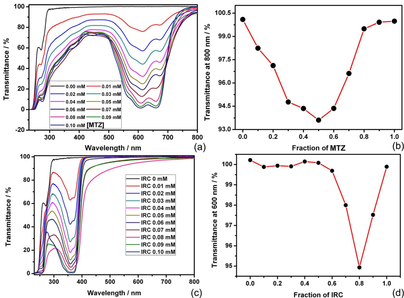
Figure 2 | (a) Optical transmittance of SC4AH–MTZ mixtures of varying fractions, while [MTZ] + [SC4AH] = 0.1 mM. (b) Dependence of the optical transmittance at 800 nm on the fraction of MTZ. (c) Optical transmittance of SC4AH–IRC mixtures of varying fractions, [IRC] + [SC4AH] = 0.1 mM. (d) Dependence of the optical transmittance at 600 nm on the fraction of IRC.
