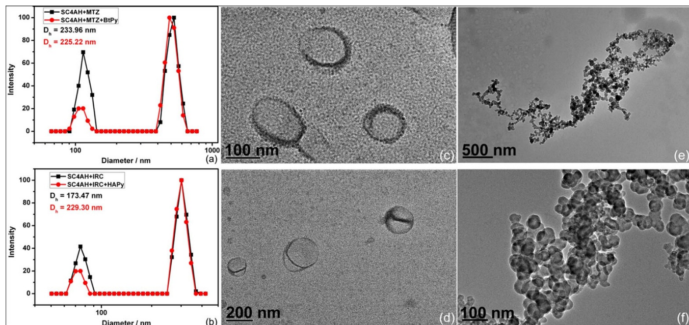
Figure 3 | Size distributions determined by scattered light intensity of (a) SC4AH–MTZ coassembly with and without BtPy (0.04 mM) and (b) SC4AH–IRC coassembly with and without HAPy (0.01 mM) measured by DLS. TEM images of (c, d) SC4AH–MTZ coassembly and (e, f) SC4AH–IRC coassembly.
