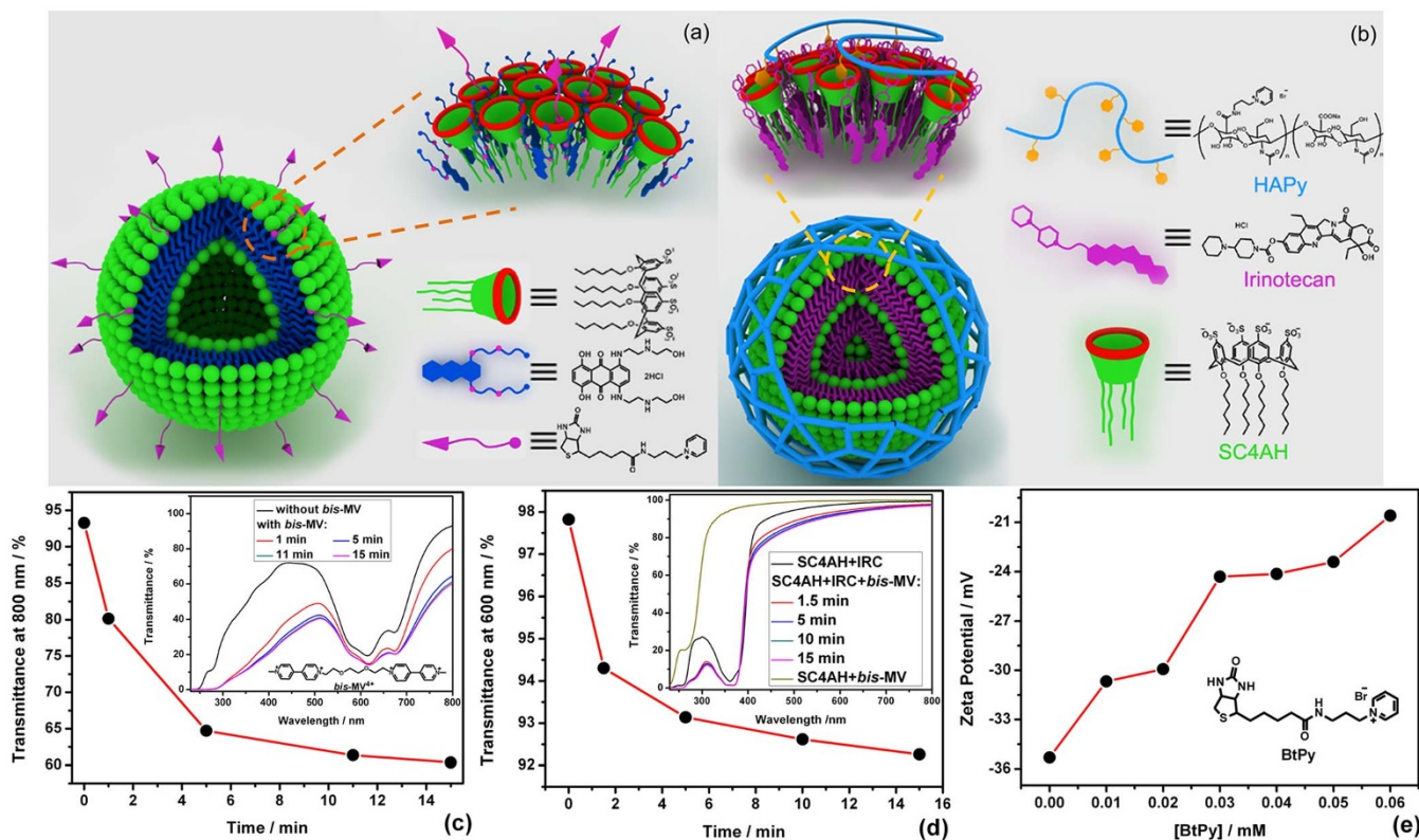
Figure 4 | Schematic illustrations of (a) SC4AH–MTZ coassembly and (b) SC4AH–IRC coassembly. (c) Dependence of the optical transmittance of SC4AH–MTZ coassembly at 800 nm on time in the presence of bis-MV (0.04 mM). (d) Dependence of the optical transmittance of SC4AH–IRC coassembly at 600 nm on time in the presence of bis-MV (0.02 mM). [IRC] = 0.08 mM, [SC4AH] = 0.02 mM. (e) Dependence of the zeta potential of SC4AH–MTZ coassembly on BtPy concentration.
