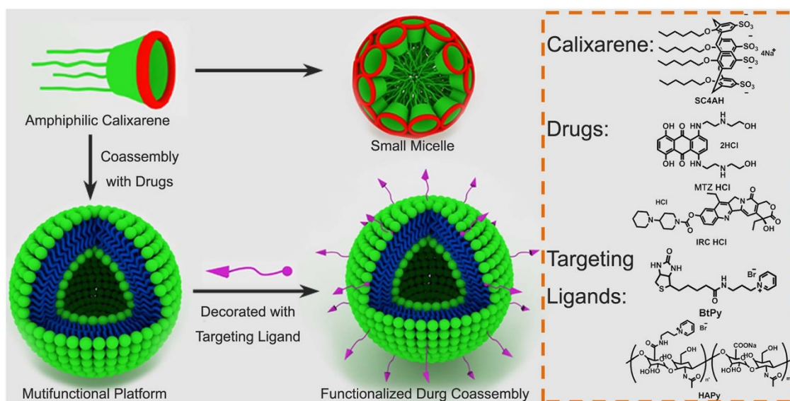
Figure 1 | Functionalization protocol of the “drug chaperone” strategy and chemical structures of anticancer drugs (IRC and MTZ), SC4AH and targeting ligands (HAPy and BtPy).
