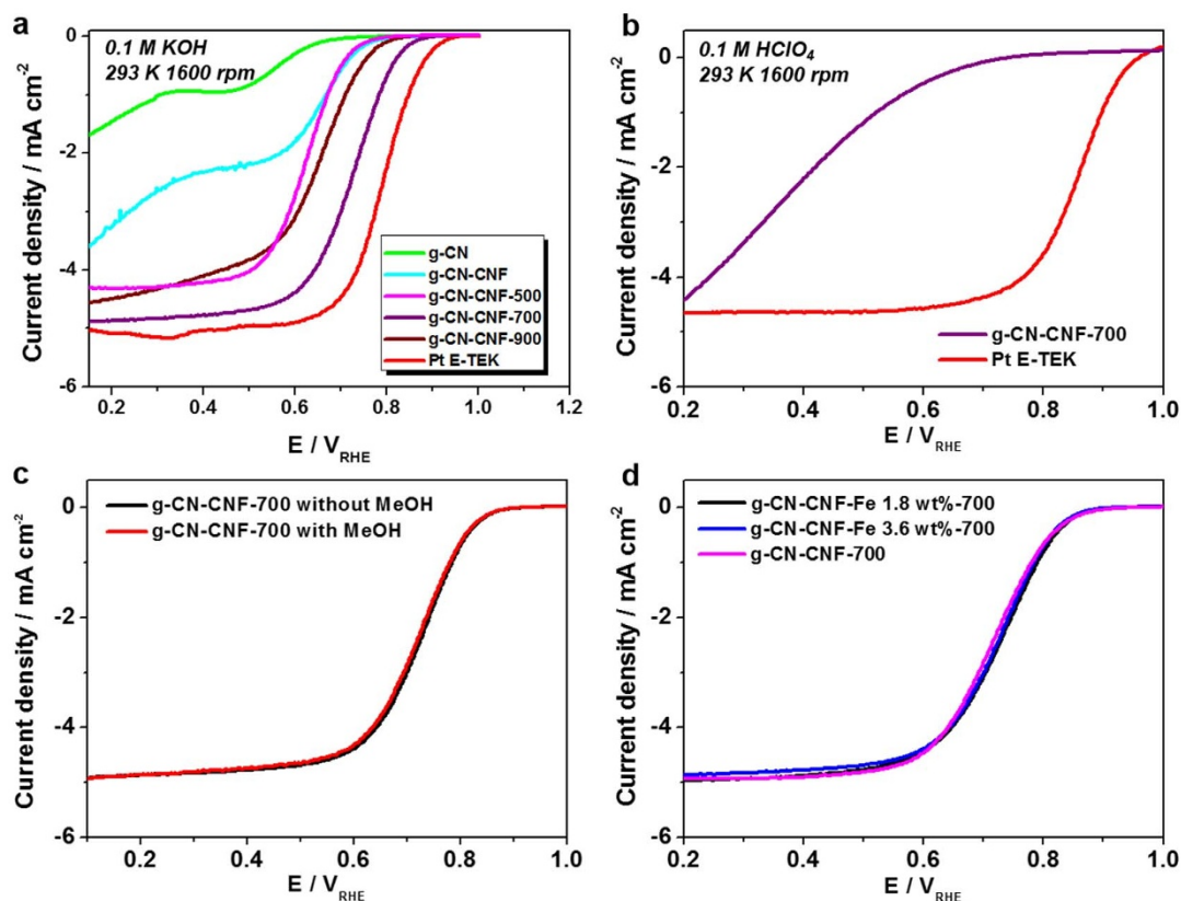
Figure 5 | Electrochemical characterization of g-CN-CNF. (a) Linear sweep voltammograms (LSVs) on RDE at 1600 rpm under 293 K of (a) g-CN-CNF pyrolyzed at various temperature in O_2 saturated 0.1 M KOH solution, (b) g-CN-CNF-700 in O_2 saturated 0.1 M HClO_4 solution. (c) g-CN-CNF-700 with/without methanol, (d) g-CN-CNF-700 with/without metal.
