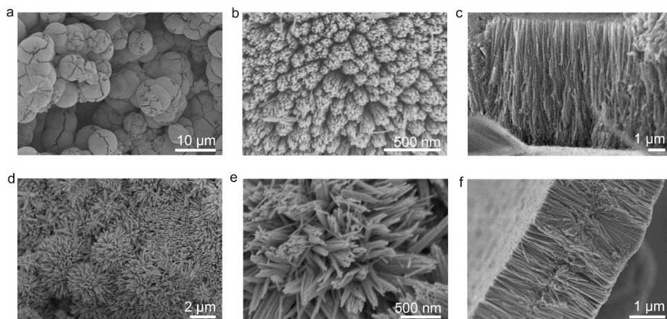
Figure 5 | Confined synthesis of \text{TiO}_2 nanowires on arbitrary substrates by using 0.3 mL of \text{TiCl}_3 solution and 15 g of lauric acid in atmospheric glass vessel at 150^\circ\text{C} for 12 h. (a) and (b) silicon substrate, (c) FTO glass, (d) and (e) Ti foil, (f) Teflon substrate.
