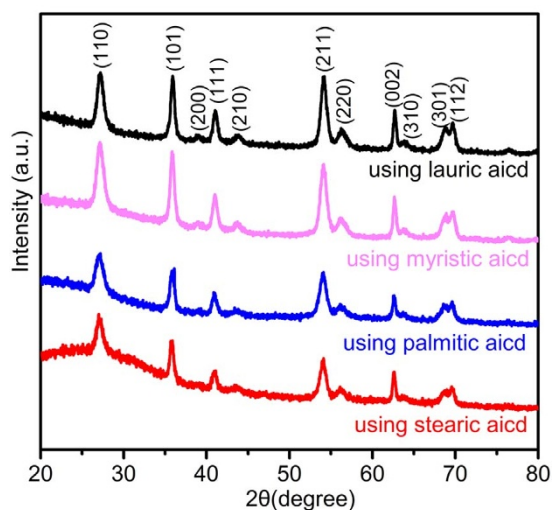
Figure 3 | XRD pattern of the TiO 2 nanowires fabricated in atmospheric glass vessel by using different saturated fatty acids at 150 °C for 12 h.
