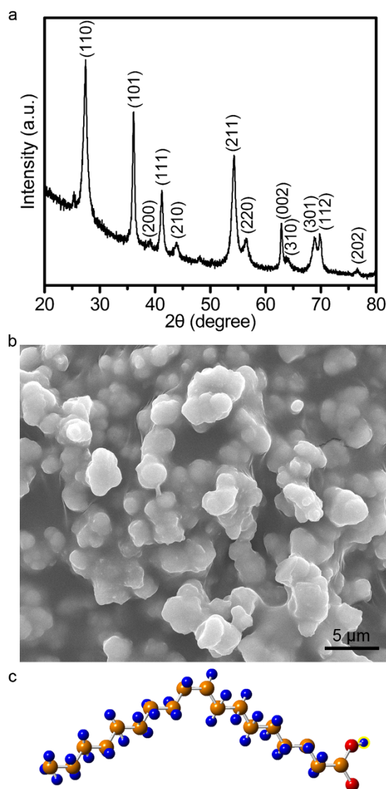
Figure 6 | The confined-synthesis of \text{TiO}_2 samples in 0.3 mL of \text{TiCl}_3 solution and 15 g of oleic acid in atmospheric glass vessel at 150^\circ\text{C} for 12 h. (a) XRD measurement. (b) FESEM images. (c) Schematic illustration for molecular structure of oleic acid. Here, the yellow, blue, and red balls represent C, H, and O atoms, respectively.
