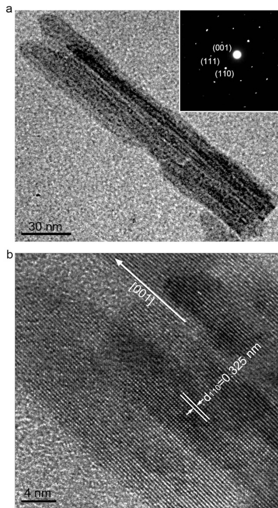
Figure 4 | Representative TEM results of TiO 2 nanowires produced with 0.3 mL of TiCl 3 solution and 15 g of lauric acid in atmospheric glass vessel at 150 °C for 12 h. (a) TEM image and corresponding SAEDs of nanowires. (b) HRTEM image of the TiO 2 nanowires.
