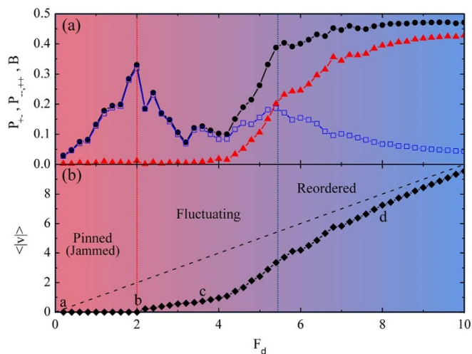
Figure 2 | (a) P_{+-} (blue squares), the fraction of dipolar walls, vs F_d has a peak just below yielding. P_{-,-,+} (black circles), the fraction of uni-polar walls, passes through a plateau when the polarized wall state forms. B (red triangles) is a measure of the net Burgers vector in the walls. (b) The average absolute value of the dislocation velocity \langle |v| \rangle (solid lower curve) vs F_d . The upper dashed curve shows \langle |v| \rangle for non-interacting dislocations. Points a, b, c, and d indicate the F_d values illustrated in Fig. 1.
