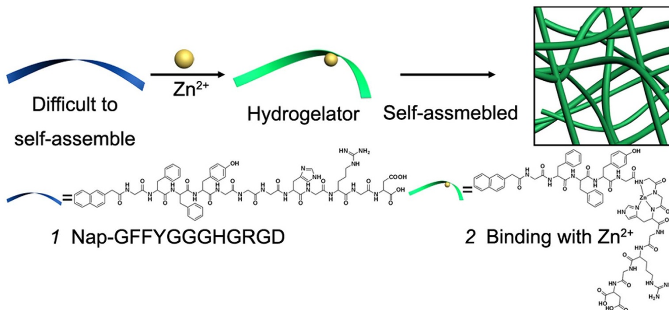
Figure 1 | Chemical structure of Zn 2+ binding peptide and schematic diagram of it binding with Zn 2+ and self-assembling into hydrogel. Blue ribbon and green ribbon stand for peptide before and after binding with Zn 2+ , respectively.
