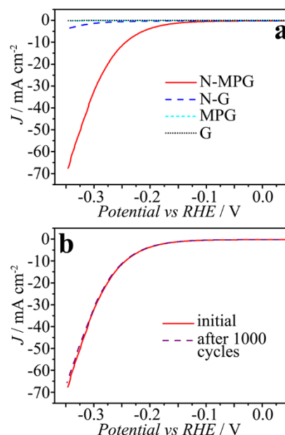
Figure 6 | HER activities of different electrocatalysts. (a) Polarization curves of N-MPG electrode, along with pure MPG, nitrogen-doped pristine graphene (N-G) and pristine graphene (G) for comparison; (b) Stability test of N-MPG through potential cycling. The scan rate is 5 \text{ mV s}^{-1} in 0.5 M H_2SO_4 .
