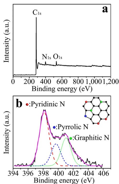
Figure 5 | XPS characterization of MPG. (a) XPS spectrum of N-MPG; (b) high-resolution N_{1s} spectrum of N-MPG. The insert in (b) shows the schematic structure of nitrogen bonding configurations.
