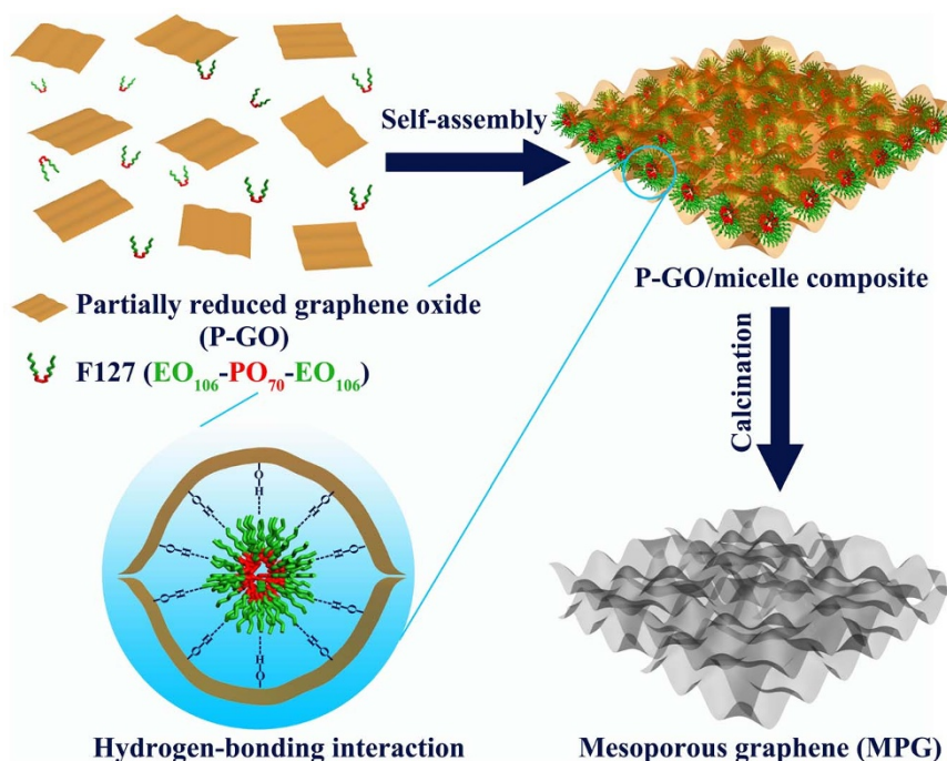
Figure 1 | Schematic illustration for preparing mesoporous graphene. Self-assembly of partially reduced GO and F127 micelles, followed by calcination to obtain MPG.
