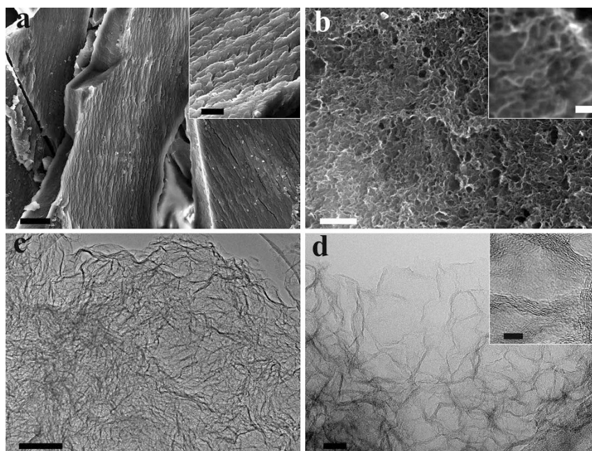
Figure 2 | Morphology and structure of MPG. (a) SEM images of MPG; (b) HRSEM images of MPG; (c) and (d) TEM images of MPG; insert of (d) is HRTEM image.
