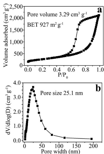
Figure 3 | Nitrogen adsorption-desorption characterization of MPG. (a) Nitrogen adsorption-desorption isotherms of the MPG; (b) the pore size distribution of the MPG.
