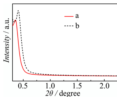
Figure 4 | The low-angle XRD patterns. (a) MPG and (b) P-GO/micelle composite.
