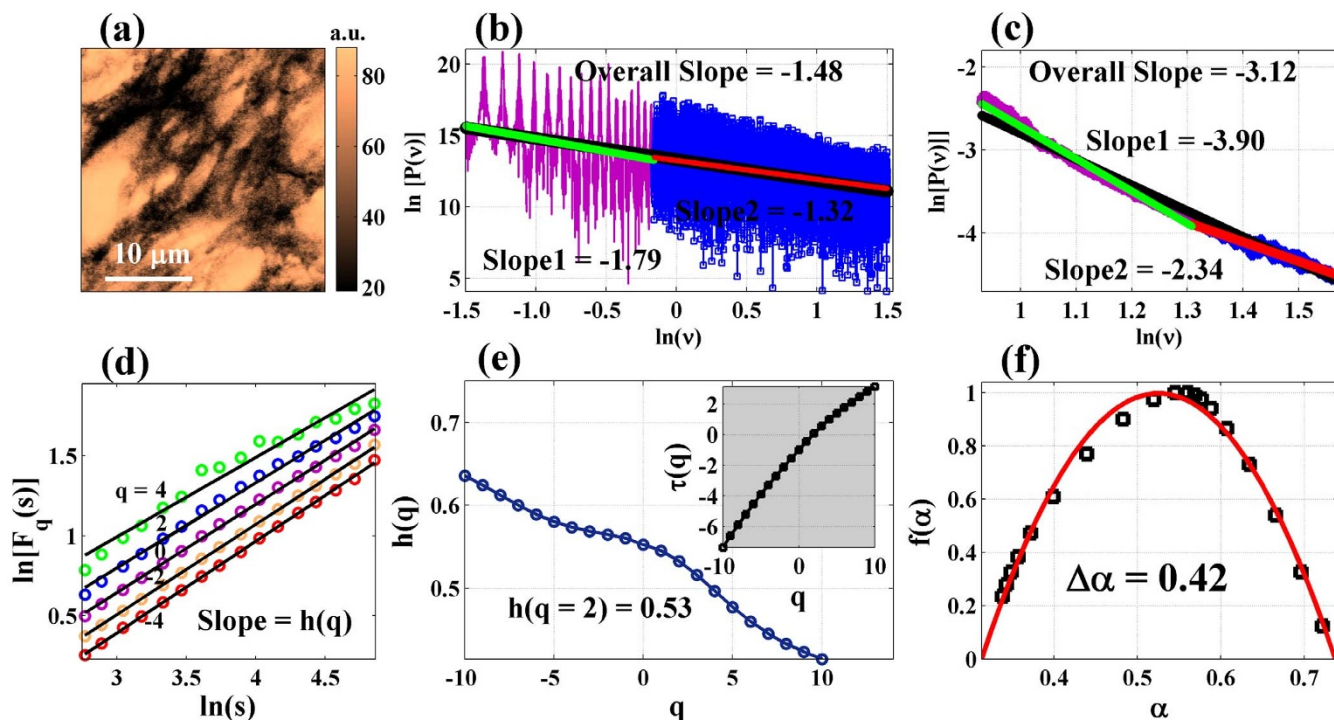
Figure 1 | Evidence of multifractality in the spatial variation of tissue RI. (a) DIC image of typical Grade I precancerous human cervix (connective tissue slice). (b) Fourier power spectrum of the generated 1D RI fluctuation series (shown in natural logarithm scale). Fitting at two selected v -ranges (lower (green) and higher (red), respectively) and overall fitting (black) yield different values for slope (manifestation of multifractality) (c) The light scattering signal [P(v) = I(v) \times k^{-4}] recorded from the same tissue also yields multiple spectral exponents (fitting at two selected v ranges and overall fitting on the entire v range are shown). (d), (e), (f): Results of the MFDFA forward analysis on the detrended (by least square polynomial fitting) spatial index fluctuations (from the DIC image). (d) The variation of the moment ( q ) dependent fluctuation function F_q(s) with length scale s (constructed using Eq. 2). The points represent the MFDFA-derived values of F_q(s) and the lines are power law fitting. Considerable variation in the slopes of \log F_q(s) vs \log s with varying q confirms multifractality. (e) The variation of the generalized Hurst exponent h(q) (derived from the slopes of \log F_q(s) vs \log s ) and the classical scaling exponent \tau(q) (derived using Eq. 3) (inset). The points represent the MFDFA-derived values and the lines are guide for the eye (for these and all subsequent figures displaying these parameters). (f) The resulting singularity spectrum f(\alpha) (derived using Eq. 4). The points represent the derived values for f(\alpha) and the line represents the fitted data (using 2 nd order polynomial) for this and all subsequent figures displaying f(\alpha) . The value for the full width of the fitted singularity spectrum, \Delta\alpha (taken at f(\alpha) = 0 ) is noted in the figure.
