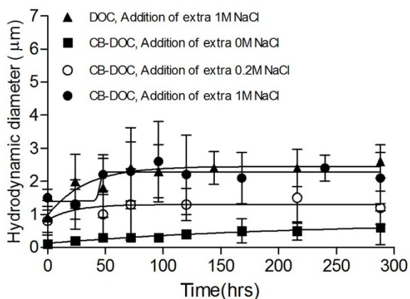
Figure 3 | Effects of NaCl on the self-assembly kinetics of DOC with/without 120 \mu\text{gL}^{-1} of CB particles in seawater. Different concentrations of NaCl added to the CB-DOC sample, including 0 M (squares), 0.2 M (open circles), and 1 M (solid circles), were monitored with DLS for over ten days.
