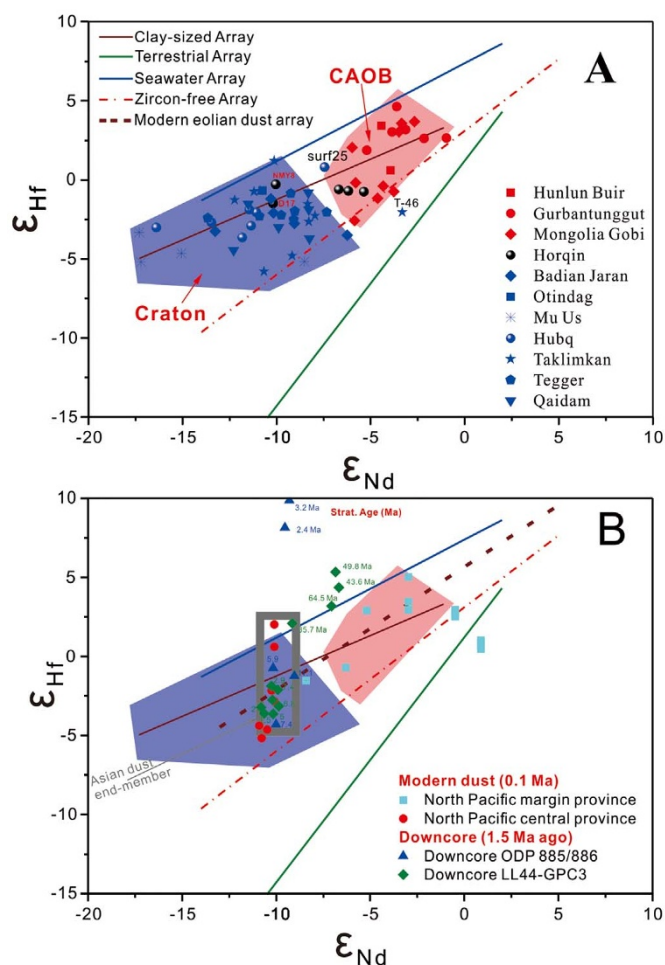
Figure 2 | The diagram for the clay-sized \epsilon_{Hf} and \epsilon_{Nd} from all major Chinese deserts and the Mongolia Gobi desert. The clay sized array is shown through the regression with all clay-sized desert Hf-Nd isotopic data: \epsilon_{Hf} = (0.45 \pm 0.04) \times \epsilon_{Nd} + (2.81 \pm 0.35) ( R = 0.80 ). The new Terrestrial Array ( \epsilon_{Hf} = 1.55 \epsilon_{Nd} + 1.21 ), Zircon-free Array ( \epsilon_{Hf} = 0.91 \epsilon_{Nd} + 3.1 ) and Seawater Array ( \epsilon_{Hf} = 0.62 \epsilon_{Nd} + 5.27 ) are from Vervoort (2011) 21 , Bayon(2009) 23 and David (2001) 48 , respectively. The \epsilon_{Hf} - \epsilon_{Nd} diagram compares the desert clays with the Asian eolian dust extracted from the North Pacific Ocean 17 .
