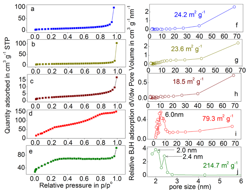
Figure 4 | Surface analysis of \text{Co}_3\text{O}_4 nanocrystals. \text{N}_2 absorption isotherms of (a) \text{Co}_3\text{O}_4 nanocubes, (b) pseudo octahedral \text{Co}_3\text{O}_4 , (c) {110} facets exposed nanosheets, (d) {111} facets exposed hexagonal nanoplatelets, and (e) {112} facets exposed nanolaminars. (f–j) are their corresponding pore size distribution, derived from absorption hysteresis of Brunauer–Emmett–Teller (BET) surface area measurement. The surface areas are listed in each subfigure from (f) to (j). The average pore sizes of hexagonal \text{Co}_3\text{O}_4 nanoplatelets and \text{Co}_3\text{O}_4 nanolaminars are given in (i) and (j).
