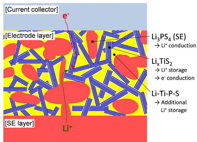
Figure 7 | Schematic diagram representing the microstructure of BMe in ASSLB. Electron and Li + ion conduction is shown. The role of each component is explained in the figure.
