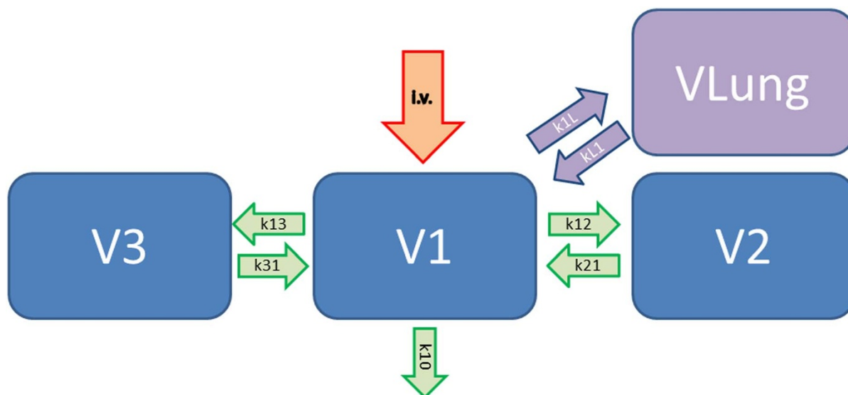
Figure 2 | 3-compartment pharmacokinetic model extended with an additional lung compartment with a volume ( V_{Lung} ) and clearance ( Cl_{Lung} ). LCC = (k_{1L} * PPC - k_{L1} * LCCO) + LCCO . LCC = Lung compartment concentration, k_{1L} = Cl_{Lung}/V_1 , PPCO = Previous Propofol plasma concentration, k_{L1} = V_{Lung}/Cl_{Lung} , LCCO = Previous lung compartment concentration, V_1 = Volume first compartment marsh model ( =0,228 * \text{patient weight m [kg]} ). V_{Lung} = Volume lung compartment, Cl_{Lung} = Clearance lung compartment.
