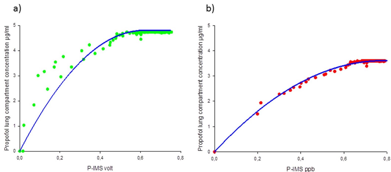
Figure 6 | Propofol lung compartment concentration. The dots are the measured propofol concentration (a) green dots: peak height [volt]), (b) red dots: concentration [ppb] versus the propofol lung compartment concentration in µg/ml. The blue line is the polynomial second order.
