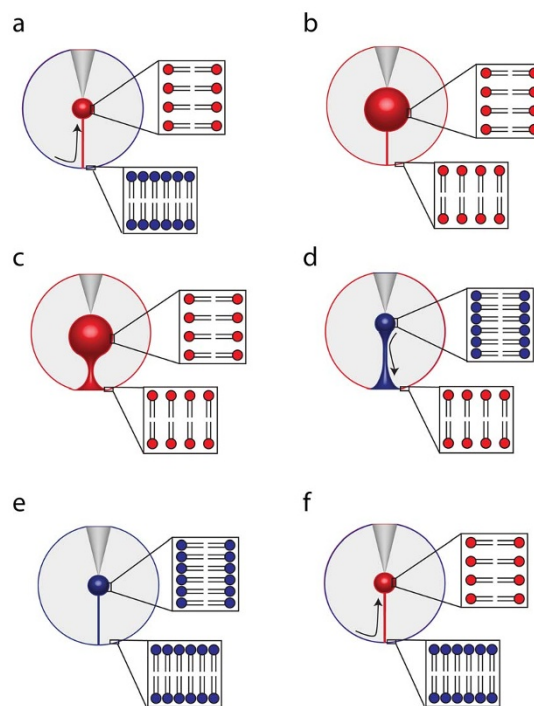
Figure 7 | Proposed model for the tension dependence in partial release mode. The blue lipids symbolize a membrane at low tension while the red lipid bilayers symbolize a membrane under tension stress. (a). The inflation of the daughter vesicle creates tension in the vesicle membrane, inducing lipid flow from the mother to the daughter vesicle. (b). At some critical size the tension between the daughter and mother vesicles equalize, stopping flow. (c). The daughter vesicle inflation continues, which requires the mother vesicle to reduce surface area to accommodate the growing daughter vesicle (d). The pore formed reduces the pressure in the daughter vesicle stopping it from growing which causes a reverse in lipid flow. (e). The surface area is minimized as the toroid collapses to a lipid nanotube (f). The closing of the pore initiates the daughter vesicle inflation and the lipid flow starts again.
