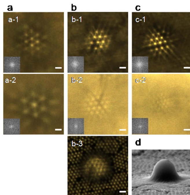
Figure 2 | Optical images of a semi-immersed microscale lens on a large object at different distance d . (a) d = 0 \mu\text{m} , two virtual images are formed. (b) d = 3.1 \mu\text{m} , a virtual image (b-1) and a real image (b-2) are observed. Image b-3 is the image of the object. (c) d = 4.1 \mu\text{m} , a virtual image (c-1) and a real image (c-2) are observed. (d) SEM image of a semi-immersed microscale lens. The large object is fabricated with the 960 nm microspheres. The lens is semi-immersed in the SU-8 resist. The scale bar is 2 \mu\text{m} .
