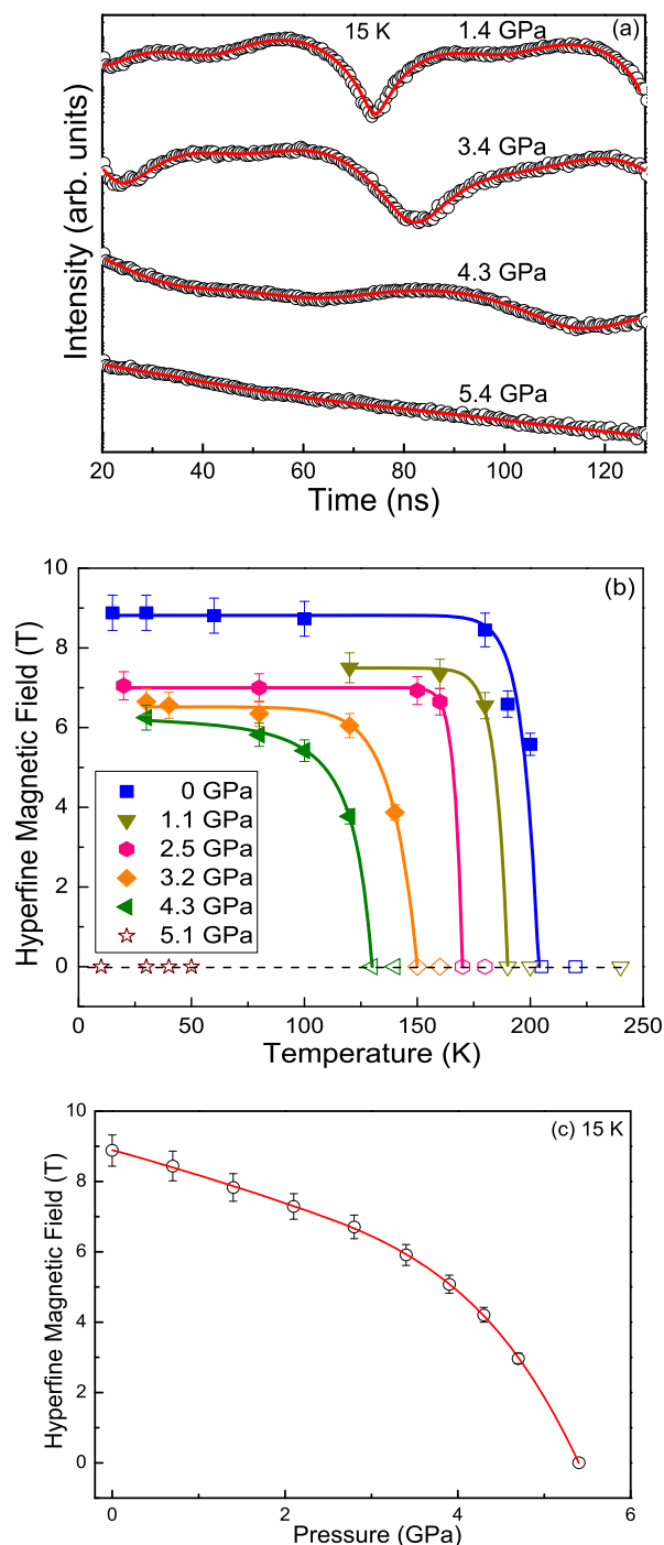
Figure 1 | (a) Representative pressure dependent SMS spectra of \text{SrFe}_2\text{As}_2 at 15 K in Ne medium. Open circles: experimental data; red solid lines: modeled spectra using CONUSS program. Quantum beats in the spectra represent the occurrence of the magnetic field and hence the AFM state, whereas the absence of the beats (flat spectral feature) is indicative of the PM state. (b) Derived hyperfine magnetic fields of the AFM \text{SrFe}_2\text{As}_2 as a function of temperature at representative high pressures. Appearance and disappearance of the magnetic fields are used to construct the magnetic PM-AFM transition as a function of P - T . Filled symbol: AFM state; open symbol: PM state. (c) Derived hyperfine magnetic fields of \text{SrFe}_2\text{As}_2 as a function pressure at 15 K.
