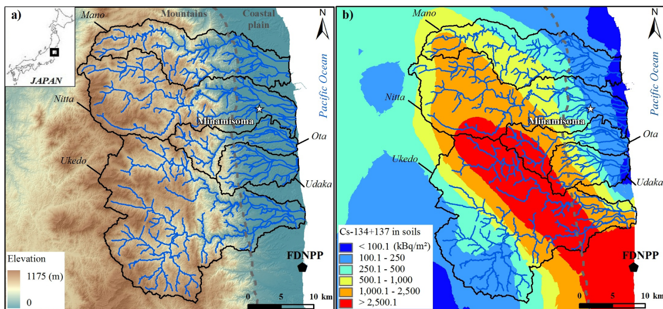
Figure 1 | Overview of the investigated contaminated catchments: (a) elevation map based on LIDAR monitoring (provided by GSI), and (b) contamination map for ^{134}\text{Cs}+^{137}\text{Cs} . This original map was created using ArcGIS 9.3 software.
