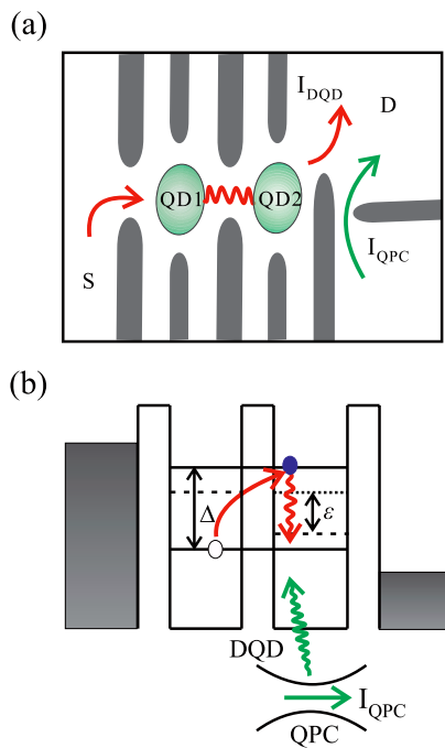
Figure 1 | The coupled DQD-QPC system. (a) Schematic diagram of a DQD coupled to two electrodes (S and D) via tunneling barriers. A QPC used for measuring the DQD electron states yields backaction on the DQD. (b) Electronic transition between two eigenstates |g\rangle and |e\rangle of the DQD (with a transition energy \Delta ) can be induced by the charge detector QPC. The energy difference \varepsilon between the two single-dot levels (dashed lines) can be varied by tuning the gate voltages.
