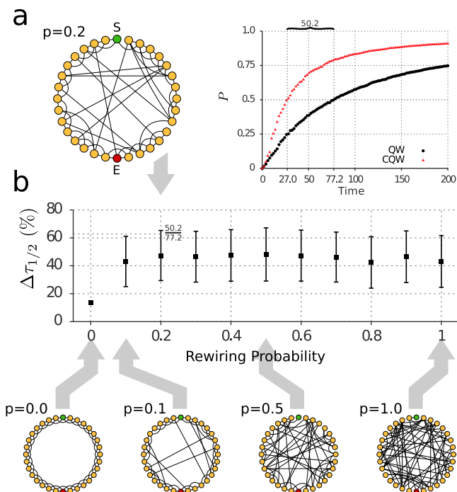
Figure 3 | Transport enhancement of the chiral quantum walk is robust across randomly generated Watts-Strogatz networks. An example of this small-world network, with rewiring probability p = 0.2 , is depicted in (a). The transfer probability P from site S to the sink connected to site E is plotted in a realization of the network. (b) shows the average enhancement of half arrival time ( \Delta\tau_{1/2} ) for different values of p .
