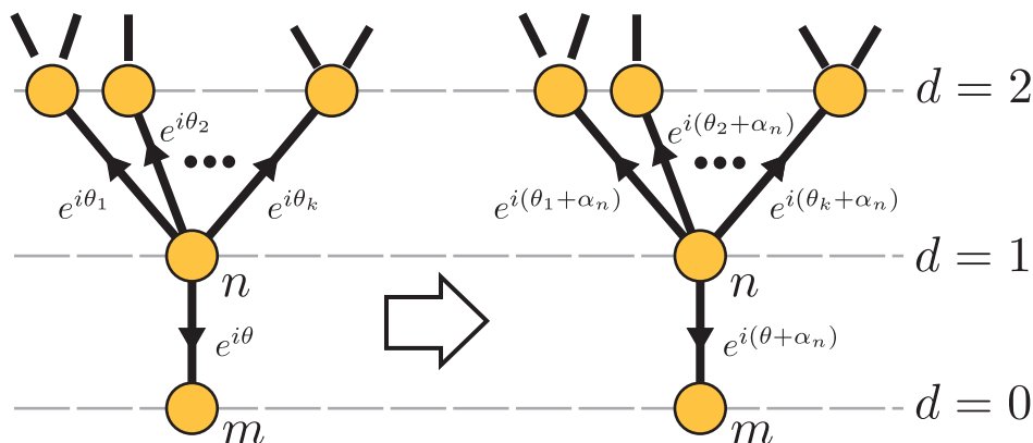
Figure 4 | Effect of the gauge transformation |n\rangle \rightarrow e^{i\alpha_n}|n\rangle on vertex n . Phases on edges can be gauge-transformed without changing the transition amplitudes, as described in the text. Here we arrange the graph as a tree rooted at d = 0 .
