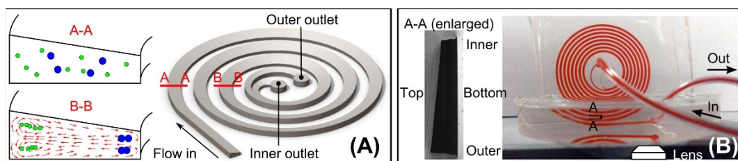
Figure 8 | (A) Schematic of a trapezoidal cross-section spiral microchannel illustrating the principle of particle focusing and trapping within the Dean vortices. (B) An actual spiral microfluidic device for side view focusing position measurement. The microfluidic channel is filled with red dye for visualization. Samples are flowed from center loops to outer loops for the measurement.
