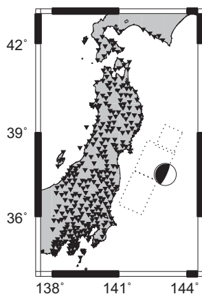
Figure 1 | 341 GPS stations in NE Japan. We use displacement time-series at 341 GEONET stations near the source region of the 2011 Tohoku megathrust earthquake, as represented by solid triangles. The beach-ball symbol shows the GCMT solution 17 . The moment magnitude is 9.1. The dashed squares illustrate the ruptured area estimated by GEONET data 18 .
