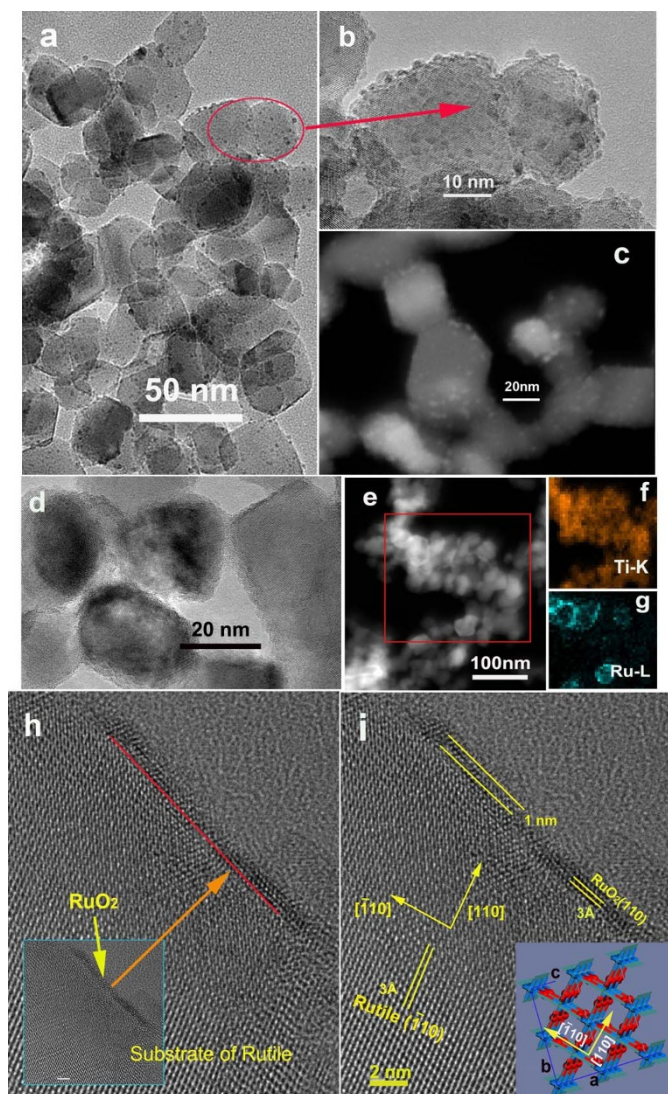
Figure 2 | Shape transformation of RuO 2 nanoparticles on the surface of P25 TiO 2 . (a–b) low and high resolution TEM images showing the uniform loading of sub-2-nm RuO 2 nanoparticles on the surface of P25-TiO 2 . (c) HAADF-STEM image showing the appearance of RuO 2 nanoparticles on TiO 2 surface. (d) TEM image showing the disappearance of the original RuO 2 nanoparticles. (e) HAADF-STEM image indicating that Ru element was preserved on the surface of TiO 2 by the bright contrast. (f–g) Element mapping results of Ti and Ru corresponding to the selected area in (e). (h) and (i) Spherical aberration-corrected high-resolution transmission electron microscopy images illustrating an epitaxial island of RuO 2 on the rutile(110) surface, with a thickness of ~1.0 nm. The inset in (f) is the orientation of rutile <110> directions.
