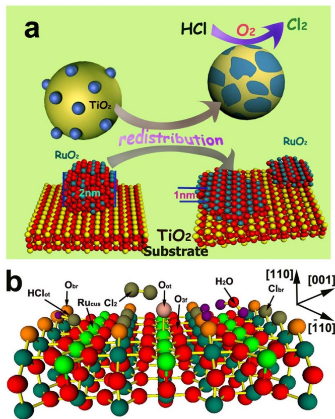
Figure 3 | (a) Schematic diagram illustrates the evolution of RuO 2 catalysts on the surface of TiO 2 from sub-2-nm nanoparticles to lattice-matched atomic-level epitaxial layer. (b) Mechanism of the Deacon reaction over RuO 2 (110) surface based on well-studied DFT calculations.
