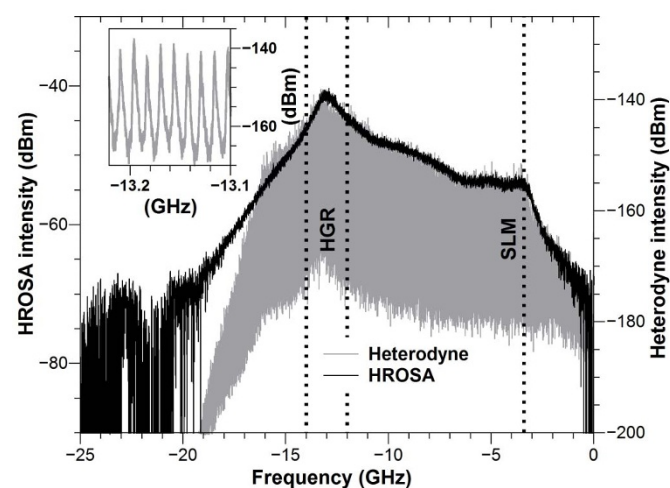
Figure 2 | Typical time averaged emission spectrum of the delayed feedback laser. The gray trace is constructed using the FFT of an entire heterodyne timetrace. The black curve is the spectrum obtained from a high resolution optical spectrum analyzer. For clarity we indicate the solitary laser mode (SLM) and the high gain region (HGR) via dotted lines. The inset presents a zoom of the heterodyne spectrum, revealing the individual cavity modes with an average width of 3 MHz.
