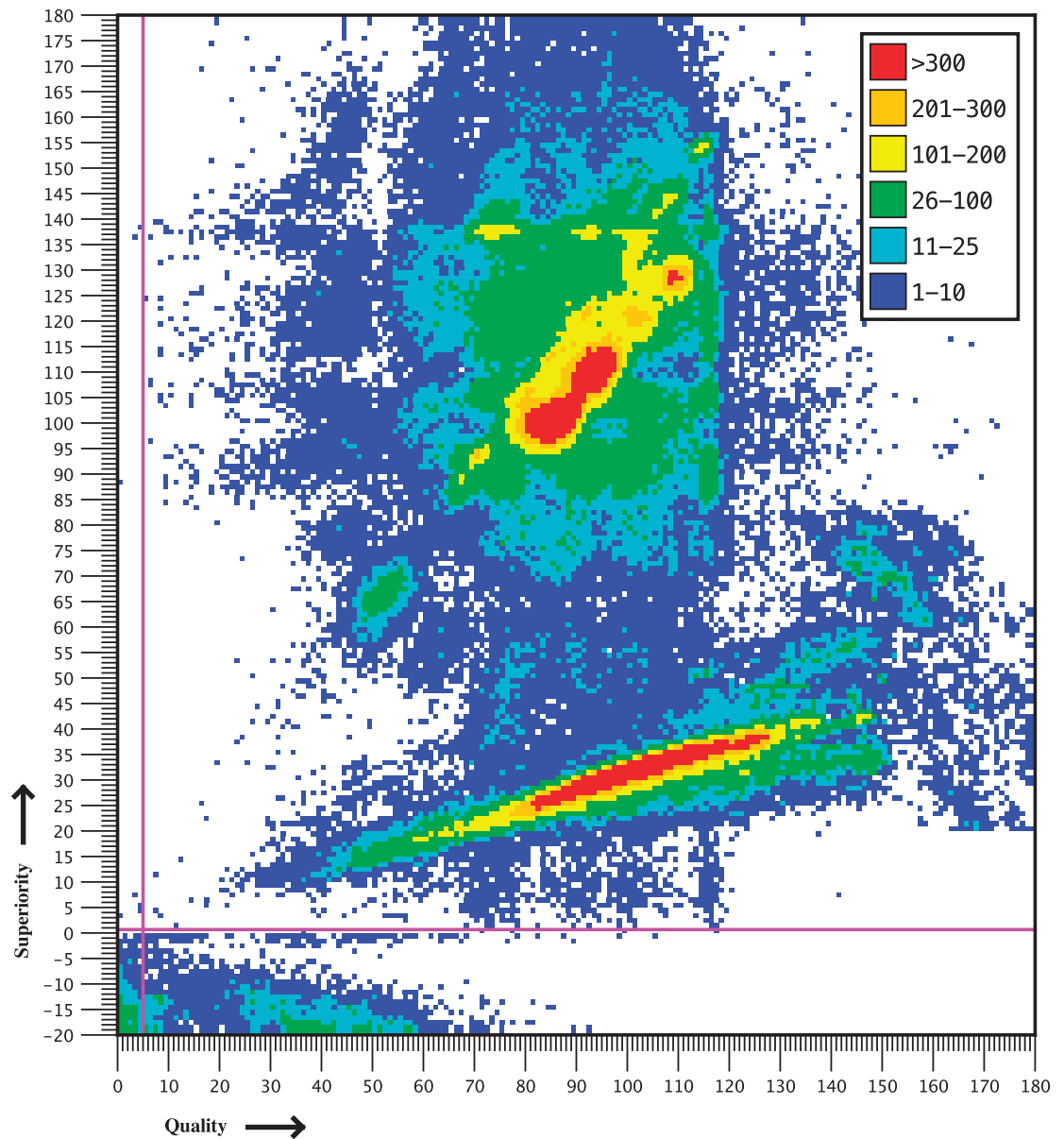
Figure 2. Distribution of accepted/rejected metazoan sequences with length \geq 95 aa.
