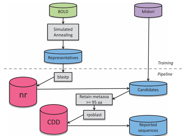
Figure 1. CO-ARBitrator data flow.
