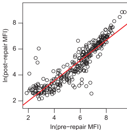
Figure 4. Correlation between \ln(\text{MFI}) values pre- and post-repair of the Luminex machine used to run the assays, based on 293 samples. The linear regression line is in red. ( R^2 0.81, F-statistic: 1306 (1, 296), P < 2.2e-16 ).
