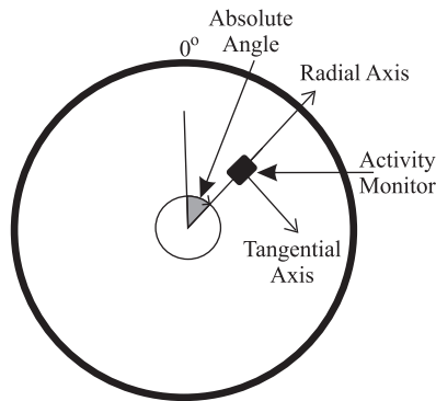
Figure 1 Demonstrating the attachment of the tri-axial accelerometer to the rear wheel of a manual wheelchair. Absolute angle of the wheel is measured from 0° to the centre of the activity monitor.
