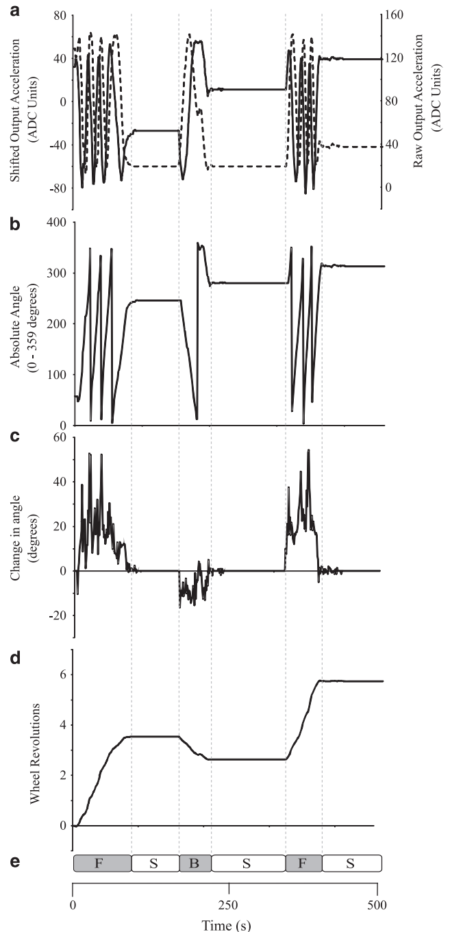
Figure 2 Graphs showing an excerpt of wheelchair propulsion. (a) Radial (solid line) and tangential (dashed line) acceleration components of the tri-axial accelerometer, (b) absolute angle of the wheel, (c) change in angle, (d) wheel revolutions of the rear wheel, (e) direction and stationary periods of the wheelchair. ADC units, Analogue to digital converted units; B, backward movement; F, forward movement; S, stationary.
