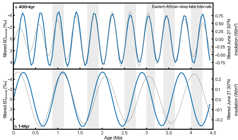
Fig. 4 Filtered leaf wax dataset compared with insolation and deep lake intervals. Gaussian filtering of \delta D_{\text{precip}} from this study (blue) and 30^{\circ}\text{N} June 21 st insolation (gray) at the 400-kyr (a) and 1-Myr (b) bands, with exact frequencies noted in Methods. Eastern African deep lake intervals from ref. 56 and ref. 35 highlighted in gray.
