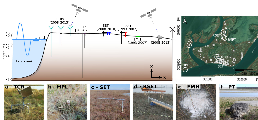
Fig. 2 Monitoring network established at San Felice salt marsh (Venice Lagoon) over the time interval of 1993–2013. The top-left panel shows a sketch of the several instruments with their reference depths and the data collection timeframes. The locations of the instruments/sensors along the marsh transect (x-axis) are for graphical purposes and do not follow the actual in situ positions. Panels a–f show the images of the monitoring instruments/sensors: a artificial trihedral corner reflectors (TCRs), b benchmarks monitored by very high-precision levelling (HPL), c and d surface elevation table apparatuses (SET and RSET), e feldspar marker horizons (FMH), and f point targets (PTs) consisting of natural radar reflectors. The geographic locations of the instruments/sensors are shown in the top-right panel (modified after 33 ). Note that FMHs are located in the same positions of the SET and RSET and the PTs are scattered over the marsh (gray squares).
