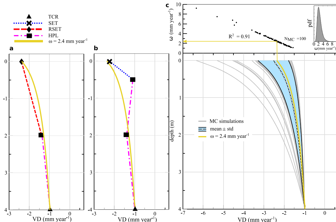
Fig. 4 Profiles of below-ground vertical dynamics from available data and modeling results. Panels a and b show the profiles obtained from data collected at the San Felice salt marsh (Fig. 3). Measurements from the 4-m-depth trihedral corner reflectors (TCRs), the high-precision levelling (HPL), the rod surface elevation tables (RSET, only panel a , and SET, only panel b ) are used to reconstruct the vertical displacements occurring at a depth range of 0–4 m. Panel c shows the below-ground vertical dynamic results of the Monte Carlo (MC) simulations ( N_{MC} = 100 model runs) assuming a prior probability distribution function for the model input accretion rate \omega \sim \text{logN}(0.84, 0.39) (top sub-panel). The best-fit simulation at the marsh surface corresponds to an input accretion rate \omega = 2.4 \text{ mm year}^{-1} .
