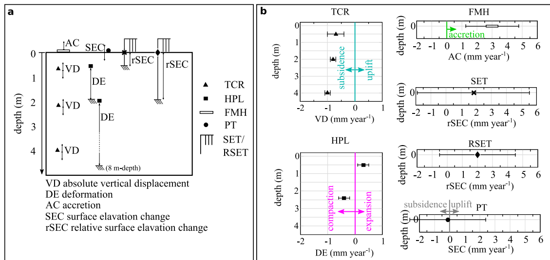
Fig. 3 Below-ground marsh deformations and accretion rates using the dataset available in the period 1993–2013 33 . Panel a shows a sketch of the available monitoring instruments (Fig. 2) with their measurement depths and types, i.e., absolute vertical displacement (VD), deformation (DE), accretion (AC), surface elevation change (SEC) and relative SEC (rSEC). Note that the sketch only shows one instrument per measurement type. In panel b , the scatter plots of the average measurement values are reported with error bars indicated their standard deviation (Table 1).
