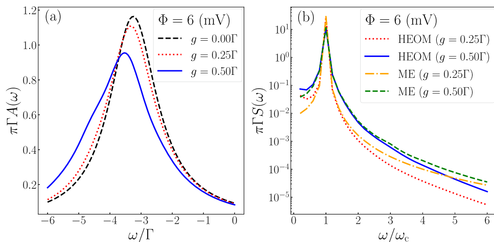
Fig. 4 Effects of the electron-cavity coupling on the spectra of the charge and cavity system. In a , the black dashed, red dotted, and blue solid curves represent the density of states A(\omega) for the charge-cavity coupling strength g at 0, 0.25\Gamma , and 0.5\Gamma , respectively. The resonance in the density of states of the charge system is reduced and shifts towards lower energies as g increases. In b , we plot the power spectral density S(\omega) of the cavity and uses two different methods [HEOM (red dotted and blue solid curves for g at 0.25\Gamma and 0.5\Gamma , respectively) and perturbative master equation (abbreviated as ME, which is represented by orange dash-dotted and green dashed curves for g at 0.25\Gamma and 0.5\Gamma , respectively)] to describe the interaction between the cavity and the bosonic reservoir. Both approaches show a single peak at \omega = \omega_c for g \in (0, 0.5] . The Born-Markov approximation used to derive the ME may result in an inaccurate estimation of the magnitude of the S(\omega) compared to the HEOM, especially in the high-frequency range.
