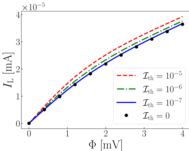
Fig. 6 Convergence of the electronic current with respect to the importance threshold. Here, we consider the parameters setting in example 1 (see Table 1) and show the electronic current I_L (from the left-hand side fermionic reservoir into the system) as a function of bias voltage \Phi where the red dashed, green dash-dotted, blue solid curves, and black dots correspond to the importance threshold \mathcal{I}_{\text{th}} at 10^{-5} , 10^{-6} , 10^{-7} , and 0, respectively. The values of electronic current converge when \mathcal{I}_{\text{th}} = 10^{-7} , which reduces the number of ADOs from 396,607 ( \mathcal{I}_{\text{th}} = 0 ) to 49,713, as shown in Table 3.
