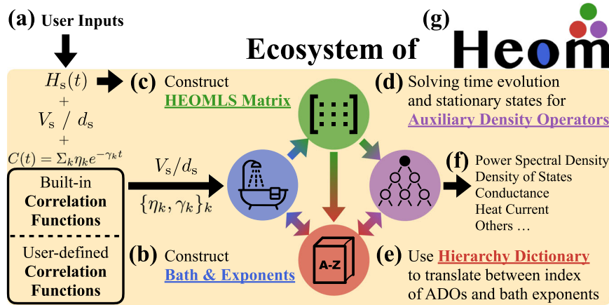
Fig. 1 The ecosystem of the HierarchicalEOM.jl package. a Users should specify the system Hamiltonian H_s(t) , coupling operators ( V_s or d_s ), and the bath correlation function C(t) . For the exponent \{\eta_k, \gamma_k\} , users can either specify the physical parameters characterizing the spectral density of the bath by built-in functions, or directly providing a list of exponents. b Construction of the bath-object which includes the system coupling operator and a list of exponents characterizing the bath correlation function. c Construction of the HEOM Liouvillian superoperator (HEOMLS) matrix \hat{\mathcal{M}} which defines the hierarchical equations of motion from the system Hamiltonian and the bath-objects. d Computation of the dynamics and stationary states for all auxiliary density operators using \hat{\mathcal{M}} . e The hierarchy dictionary translates the index of each ADO into the corresponding multi-index ensembles together with the exponents of the bath, and vice-versa. f The hierarchy dictionary allows a high-level interpretation of the ADOs to compute some physical properties. g Logo of HierarchicalEOM.jl package.
