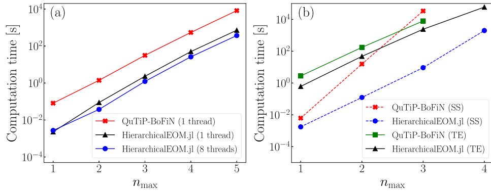
Fig. 7 Benchmark of the performance between HierarchicalEOM.jl and QuTiP-BoFiN. We consider the parameters used in example 1 (see Table 1). Note that QuTiP-BoFiN 15,83,84 currently does not support the estimation of importance for ADOs, and thus, we set \mathcal{I}_{\text{th}} = 0 here. The benchmark was done on a workstation with two Intel(R) Xeon(R) Silver 4110 @2.10GHz CPUs and 256 GB memory. The software versions were QuTiP 4.7.1, HierarchicalEOM.jl 0.1.0, Python 3.7.6, and Julia 1.8.2. The operating system was CentOS Linux 8.1.1911. In a , we show the total runtime versus truncation level n_{\max} for the construction of the HEOMLS matrices \hat{\mathcal{M}} using QuTiP-BoFiN (red crosses) and HierarchicalEOM.jl (black triangles and blue circles represent 1 and 8 threads used during the process of constructing the matrices, respectively). Note that QuTiP-BoFiN currently only supports single-thread process for the construction of \hat{\mathcal{M}} . In b , we show the total runtime versus truncation level n_{\max} for calculating the stationary states (SS), represented as dashed lines, and time evolution (TE), represented as solid lines, of the auxiliary density operators using QuTiP-BoFiN (red crosses and green squares) and HierarchicalEOM.jl (blue circles and black triangles).
