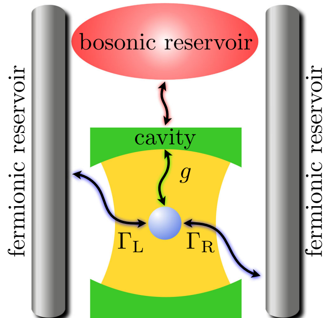
Fig. 2 Schematic illustration of a light-matter system (an electron coupled to a bosonic mode in a cavity) interacting with bosonic and fermionic reservoirs. Here, g is the coupling strength between the electron and cavity, \Delta is the coupling strength between the cavity and the bosonic reservoir, and \Gamma_L = \Gamma_R = \Gamma are the coupling strengths between the electron and its fermionic reservoirs.
