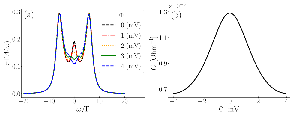
Fig. 3 The Kondo resonance from equilibrium to non-equilibrium. In a , the black dashed, red dash-dotted, orange dotted, green solid, and blue dashed curves represent the density of states A(\omega) for bias voltage \Phi at 0, 1, 2, 3, and 4 mV, respectively. One can observe that the density of states of the electronic system exhibits two Hubbard peaks and an additional central peak at equilibrium (i.e., bias voltage \Phi = 0 ). By increasing the bias voltage \Phi to non-equilibrium, the central peak is suppressed and splits into two. In b , the black curve shows the effects of the Kondo resonance on the differential conductance as a function of bias voltage \Phi . The conductance G has a peak at \Phi = 0 as the Kondo resonance acts as a transport channel for the electron.
