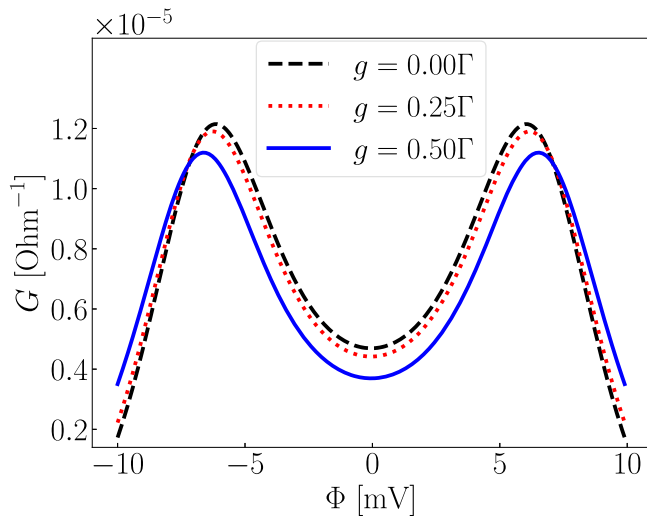
Fig. 5 Effect of the electron-cavity coupling on the conductance between the charge system and fermionic reservoirs. The black dashed, red dotted, and blue solid curves represent the conductance G for the charge-cavity coupling strength g at 0, 0.25\Gamma , and 0.5\Gamma , respectively. The conductance depends on the absolute value of the bias voltage \Phi and reaches its maximum when the average energy of the charge system is equal to the Fermi-level of one of the fermionic reservoirs, i.e., when e|\Phi|/2 = \epsilon . As the electron-cavity coupling g increases, both the conductance G and the average energy of the charge system decrease, resulting in a wider splitting of the conductance peaks.
