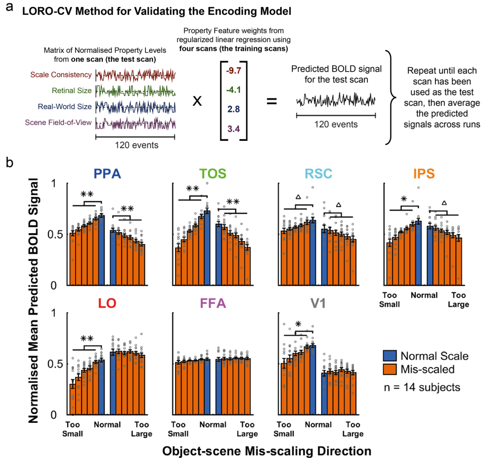
Fig. 5 Predicted BOLD signals using Encoding Model Feature Weights. a Schematic of the LORO-CV method used to validate the encoding model. b Mean predicted BOLD signals for each ROI—normalized across subjects and ROIs—for each scale consistency level, when split by object scale direction (plotted in the same manner as the GLM data in Fig. 2b). Significance tests (paired t-tests, one-tailed) were performed between the normal scale levels and the mean of the corresponding mis-scaled levels, FDR corrected for multiple comparisons across all tests and ROIs: **p < .001 , *p < .01 , \Delta p < .05 . Error bars show the SEM. Individual subject data points are overlaid on the bars as gray circles.
