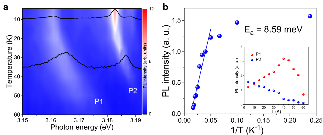
Fig. 1 Temperature-dependent micro-photoluminescence. a Temperature-dependent PL spectral mapping from graphene. Upper and bottom insets depict the PL spectra taken at 4.2 and 35 K, respectively. b The Arrhenius plot of the P2 emission. Inset depicts the integrated PL intensity of the P1 and P2 emission peaks as a function of temperature. All intensities are deduced by Gaussian fitting as shown in Supplementary Fig. 1.
