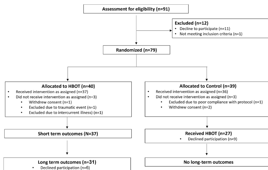
Figure 5. Patients' flowchart.
