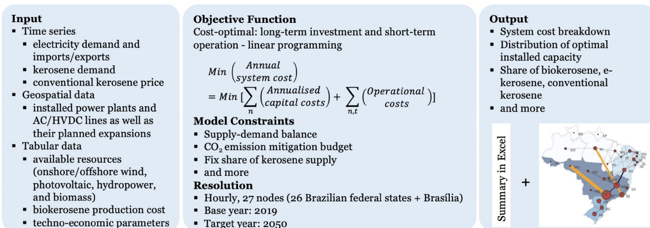
Figure 4. Overview of the PyPSA-Brazil model.
