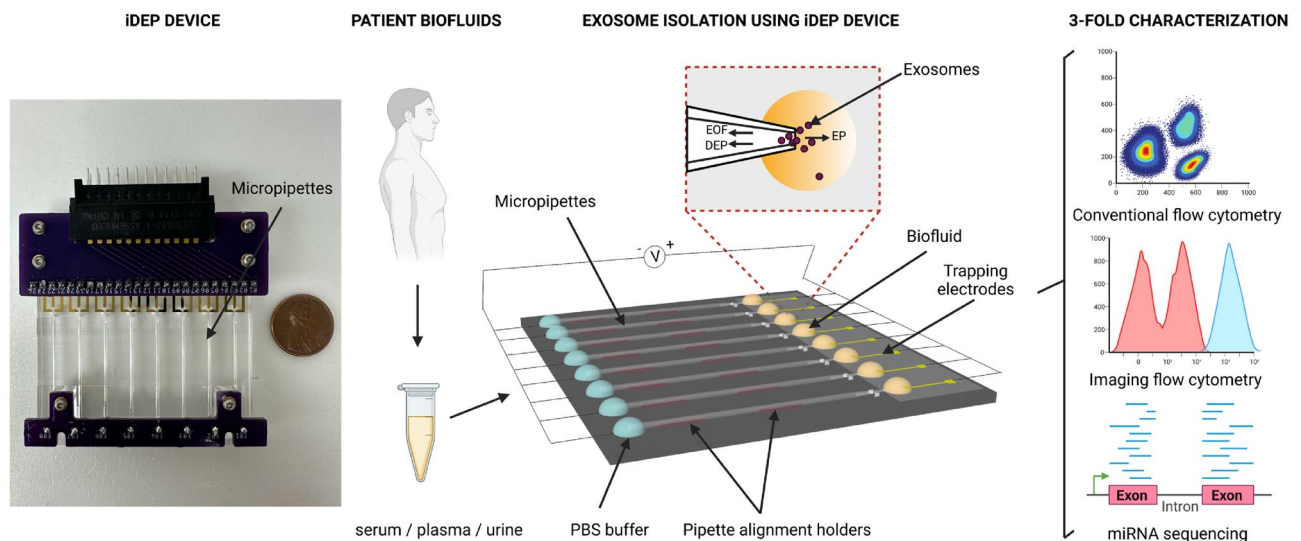
Figure 1. Device layout and graphical outline of experimental flow. Small extracellular vesicles (sEVs) were simultaneously extracted from human biofluids using the insulator-based dielectrophoretic (iDEP) device, wherein a trapping zone was created at the tip region of micropipettes by balancing the dielectrophoretic (DEP) force with two electrokinetic forces, including electroosmosis (EOF) and electrophoresis (EP). sEVs isolates were comprehensively characterized using flow cytometry, ImageStream x , and microRNA (miRNA) sequencing.
