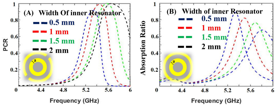
Figure 3. Trade-off due to width of inner resonator: (A) Polarization conversion ratio; (B) Absorption ratio.
