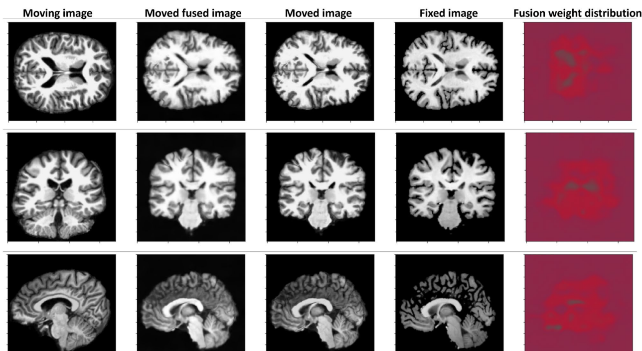
Figure 7. Sample results obtained for the implicit networks based on the proposed registration guided image fusion. Weight distribution indicates the utilization of the original image (red) and the Laplacian (green) and Gaussian (blue) filtered images. For this particular case, the average weights, Eq. (16), were equal to 0.57 (original), 0.15 (Laplacian) and 0.28 (Gaussian), indicating that all operations were utilized to process the brain image.
