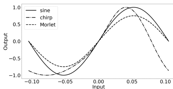
Figure 2. Sine, chirp and Morlet activation functions around 0 for \omega set to 30. For the chirp function the hyper-parameter a_\omega was set to 10.
