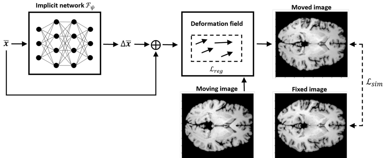
Figure 1. Scheme presenting pairwise brain image registration based on implicit neural representations. In this setting, a coordinate network is used to estimate the displacement vector \Delta\bar{x} and determine the deformation field. Note changes in the shape of the brain, gyri, and ventricles in the moved image compared to the moving image.
