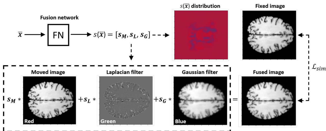
Figure 3. Scheme illustrating the proposed registration guided image fusion technique. The fused image is generated based on the weighted pixel-wise combination of the original image and images processed with the Laplacian and Gaussian filters. Weights used for image fusion are calculated using an implicit network trained to improve the registration. The weights of the distribution s(\bar{x}) = [s_M(\bar{x}), s_L(\bar{x}), s_G(\bar{x})] can be visualized with a parametric map, which pixel color intensities in the RGB space are proportional to each component of the distribution. For instance, the first weight, s_M(\bar{x}) \in [0, 1] , was mapped to [0, 255] in the red color channel. The parametric map indicates the filtering operations used to process particular image area.
