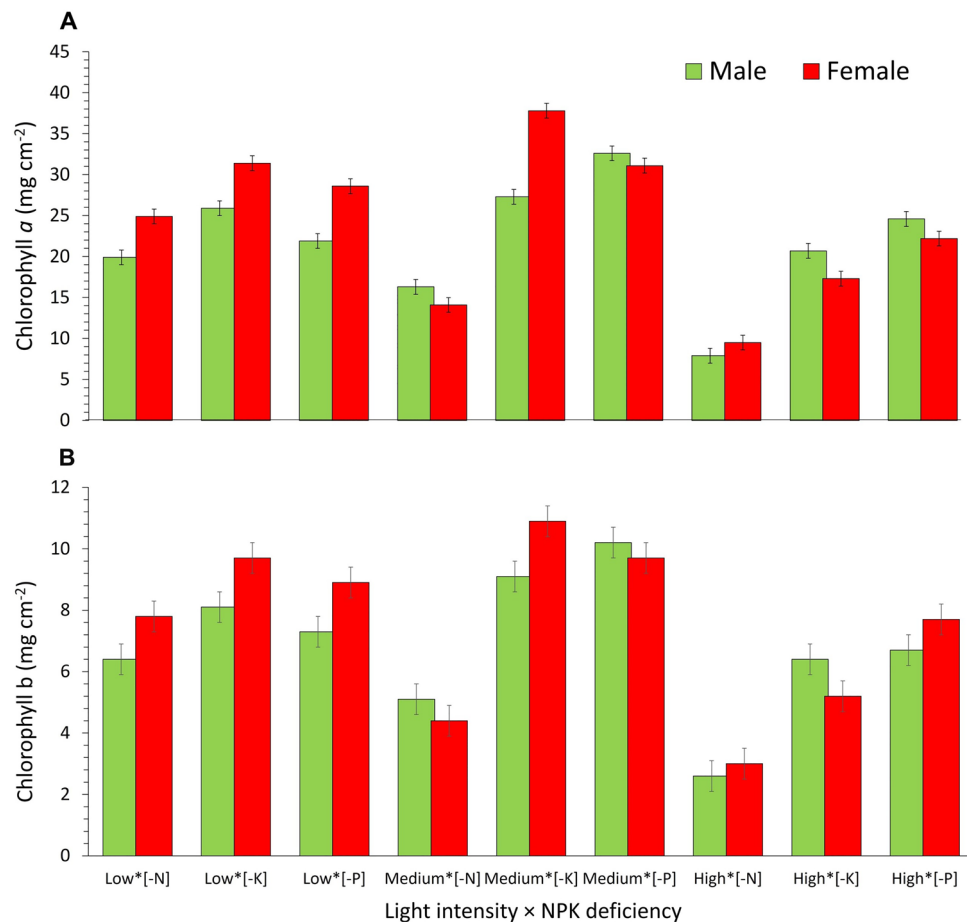
Figure 2. (A) Leaf chlorophyll a content, and (B) leaf chlorophyll b content of male and female Amaranthus palmeri plants as affected by white light intensity \times NPK deficiency averaged across 5 sampling times throughout the experimental period; Values of chlorophyll a and chlorophyll b content for male and female A. palmeri plants on the Y-axis stand for the statistically defined interaction of white light intensity \times NPK deficiency shown on the X-axis. Low, Medium, and High light intensities refer to 150 , 450 and 1300 \mu\text{mol photons m}^{-2} \text{s}^{-1} , respectively; [-N], [-K], and [-P] refer to NPK deficiency. Vertical bars represent Least Significant Difference at \alpha=0.05 .
