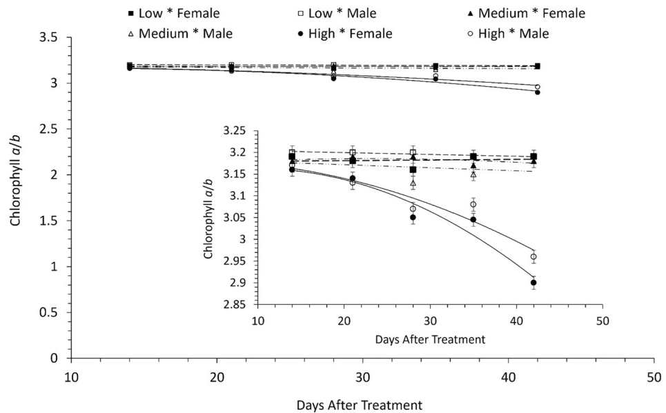
Figure 4. Effects of white light intensity on leaf chlorophyll a/b ratio as measured throughout the experimental period (DAT) for Amaranthus palmeri male and female plants and averaged across NPK deficiency treatments. The Y-axis, in the inset figure, has been rescaled to improve the readability of the figure. Squares, in the inset figure, represent the chlorophyll a/b (Chl a/b ) ratio in male plants (open squares), and in female plants (closed squares) both under low light intensity ( 150 \mu\text{mol photons m}^{-2} \text{s}^{-1} ) (see dashed line). Open triangles are for the data from the male plants, and closed triangles are for female plants, both under medium light intensity ( 450 \mu\text{mol photons m}^{-2} \text{s}^{-1} ) (long dashed line with dots). The Chl a/b ratio under high light intensity ( 1300 \mu\text{mol photons m}^{-2} \text{s}^{-1} ) (solid line) is shown for both the male (open circles) and the female (closed circles) plants. Vertical bars represent LSD = Least Significant Differences at \alpha = 0.05 .
