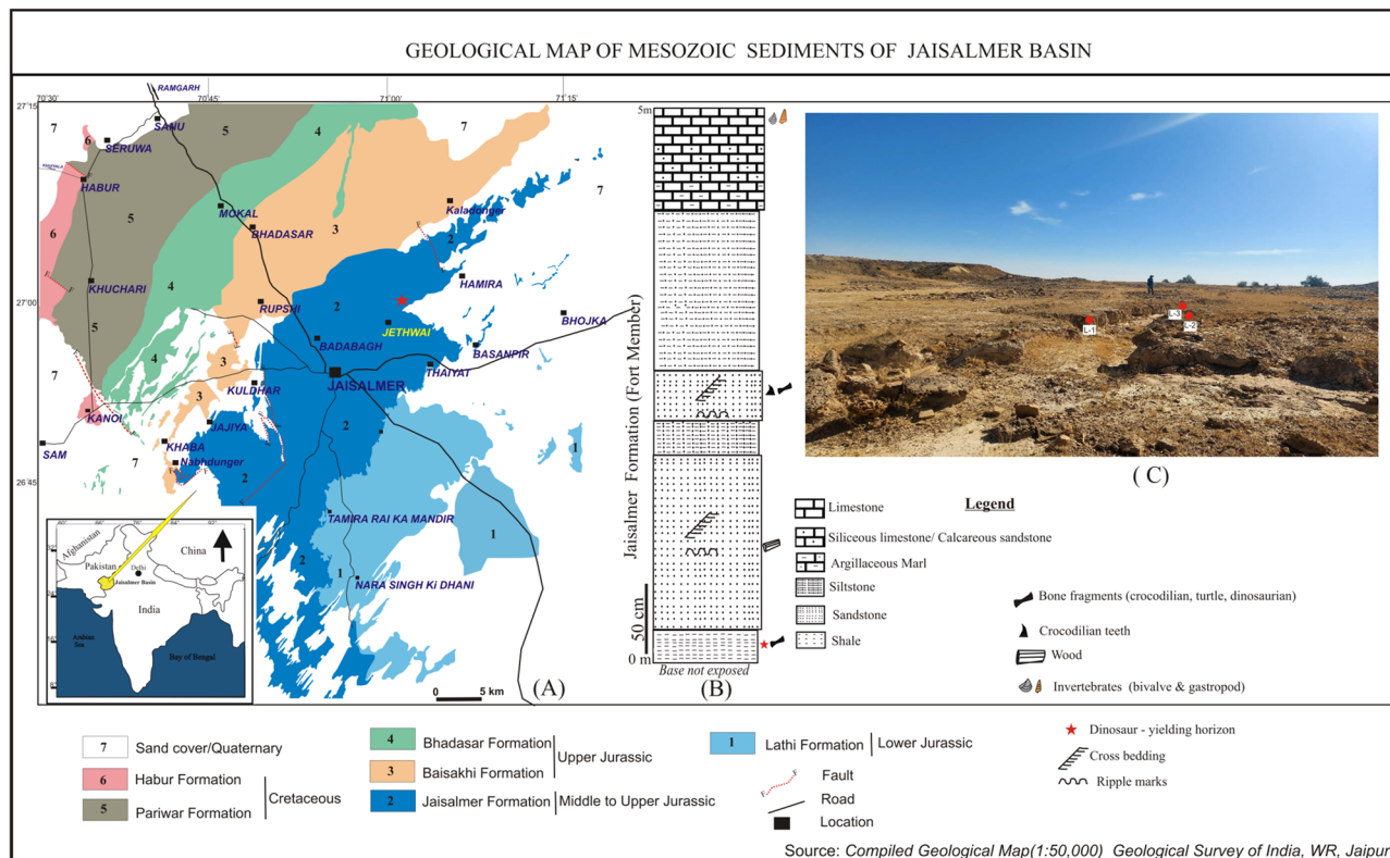
Figure 1. Geological map of Jaisalmer Basin showing (a) the fossil locality; (b) stratigraphic column showing the position of the dinosaur fossil yielding horizon; (c) photograph of the fossil site. The map and stratigraphic column were drawn by K.K. using CorelDRAW 2019 (Version number: 21.0.0.593, URL link: http://www.corel.com/en/ ).
