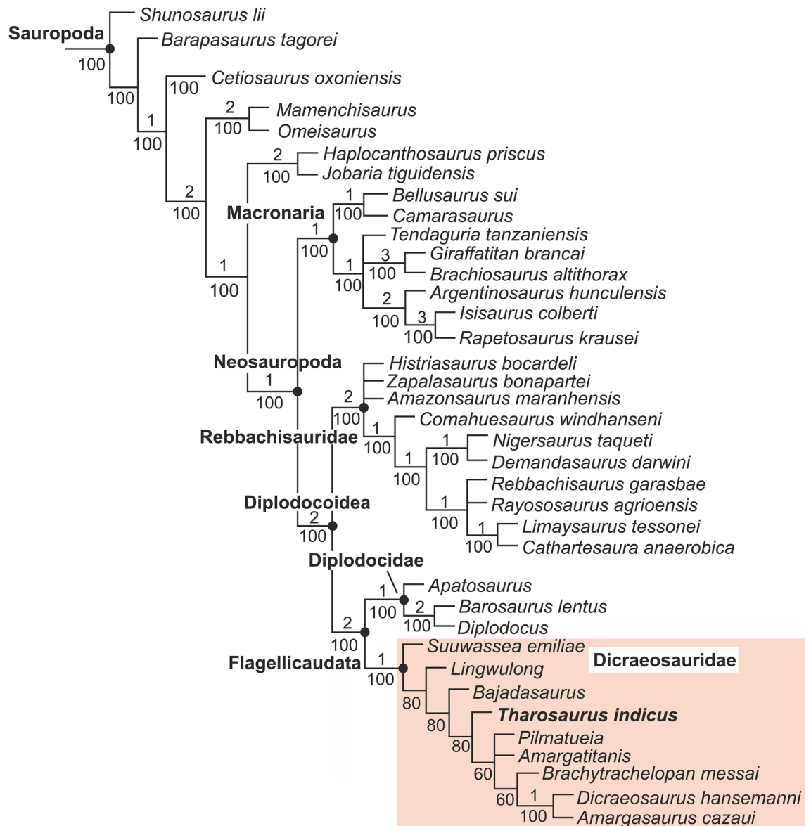
Figure 6. Phylogenetic position of Tharosaurus indicus gen. et sp. nov. (RWR-241) in 50% majority-rule tree. Clade Dicraeosauridae shaded in pink. Numbers above nodes indicate Bremer support values.
