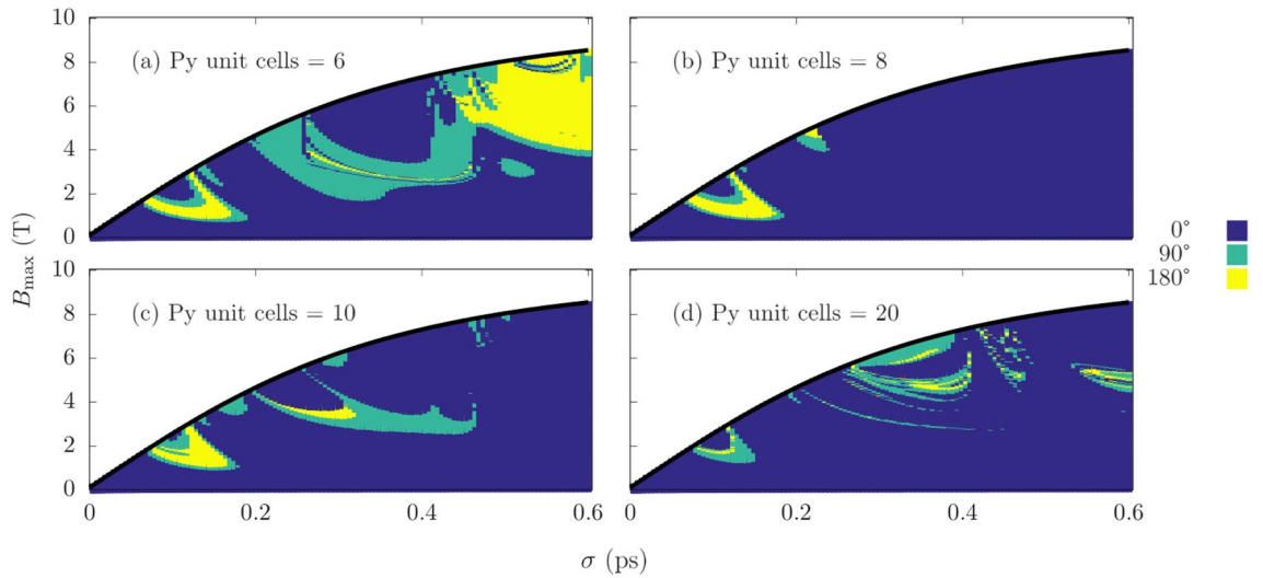
Figure 5. Magnetization reversal using a THz pulse for an interface exchange of 5.0 \times 10^{-21} J with (a) 6, (b) 8, (c) 10 and (d) 20 unit cells of Py at T = 0 K. Turquoise and yellow are regions of 90^\circ and 180^\circ switching respectively.
