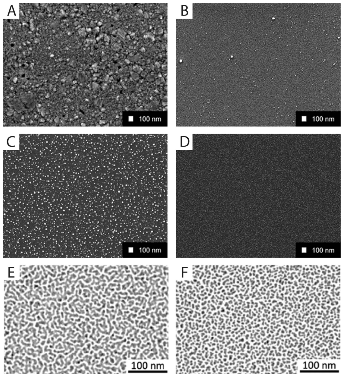
Figure 2. Exemplary electron microscopy images of continuous nanoscale films (A, B) and nanopatches (C–F). (A) SEM top view of 50 nm Ag, (B) SEM top view of 50 nm Cu, (C) SEM top view of Ag nanopatches sputtered for 60 s, (D) Ag & Pt nanopatches co-sputtered for 60 s, (E) TEM image of Ag & Cu nanopatches co-sputtered for 60 s on a TEM grid, (F) Cu on Ag nanopatches sequentially sputtered for 60 s on a TEM grid. (E, F) taken from reference 18 .
