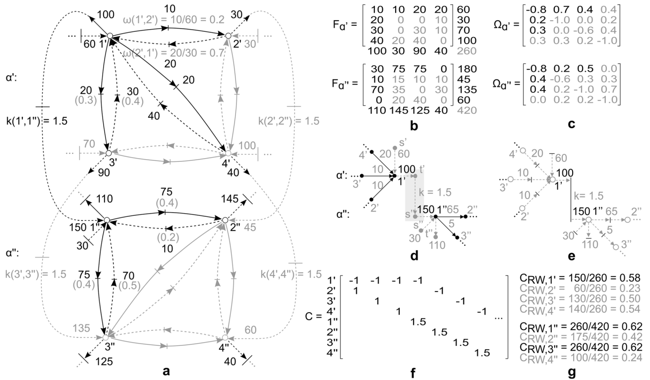
Figure 5. Simplified illustration of multilayer flow network (proxy), equivalent to the dataset of U.S. GDP by industry 54 . (a) Illustrative multilayer flow network interpretation, corresponding to dataset 54 . Nodes correspond to industries, while arcs and links correspond to economic activity (cross-industry and cross-layer network flow). Conversion coefficient k refers to a proportion defined with respect to e.g., rate of return, where layers \alpha' , \alpha'' correspond to years (note that the network could be represented in compact form as well). Rate of transfer arc weights \omega are derived from supply and cross-industry network flow. Note that a node (e.g., node 1' ), participates in domestic output and supply of commodities required by other industries (expressed in monetary terms), where total supply relates to node potential. The generated output participates, furthermore, in value added and capital carried over to the next time instance (i.e., node 1'' ). (b) Illustration of cross-industry network flow matrix F , corresponding to dataset 54 (as derived from the corresponding manual “Concepts and Methods of the U.S. Input-Output Accounts”, 2009 54 ). The dataset consists of domestic supply (rows) and use (columns) of commodities by industry (intermediate use of commodities, net of contributions and subsidies). Note that 53 relates total use, as opposed to total supply, to node potentials. (c) Compartmental weight matrix \Omega , derived from rate of transfer arc weights \omega . Note that \sum_{r^i, u^i \neq r^i} \omega(u^i, r^i) \neq 1 (see weight matrix \Omega diagonal) for some nodes (i.e., nodes \{1', 3', 1'', 2''\} ), as some funds get reinvested over time or further external investments are introduced (see flow matrix F diagonal). (d) HFN multilayer flow network excerpt (incident with nodes \{1', 1''\} ), as derived from panel b. (e) Petri net equivalent of HFN multilayer flow network excerpt incident with nodes \{1', 1''\} . (f) Incidence (coupling) matrix C , encoding intra-layer and inter-layer relationships, corresponding to network in panel a. Note that weights ( Pre, Pos ) in the Petri net equivalent, are 1 for intra-layer (identity), and k for inter-layer conversion. (g) Example of flow based random walk node betweenness centrality CRW derivation, for nodes \{1', \dots, 4''\} .
