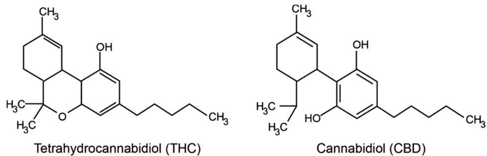
Figure 1. Chemical structures of THC and CBD.
