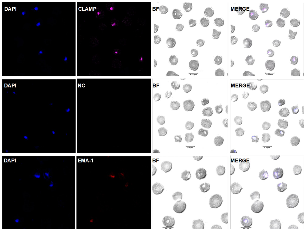
Figure 3. CLAMP is expressed in the intra-erythrocytic stages of T. equi development. Confocal microscopy images showing expression of CLAMP in T. equi infected erythrocytes. The first row shows expression of CLAMP by T. equi gamonts. Parasite nuclei are stained in blue with DAPI, and CLAMP is stained in magenta. The second row shows infected erythrocytes incubated with pre-immunization serum (negative control) and it shows lack of staining indicating test specificity. The third row indicates expression of EMA-1 (positive control (PC)) by intra-erythrocytic parasites. In all cases, BF refers to brightfield panels.
