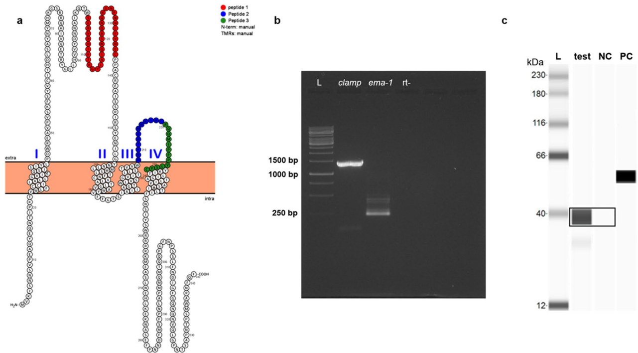
Figure 1. T. equi CLAMP contains immunogenic epitopes, and the gene is transcribed and expressed by T. equi merozoites. (a) CLAMP's transmembrane topology as predicted and annotated by Phobius and Protter algorithms, respectively. Peptides 1, 2 and 3 indicate the protein's predicted immunogenic peptides. (b) A 1% agarose gel showing amplified clamp transcript at ~1226 bp. The T. equi equine merozoite antigen-1 ( ema-1 ) transcript was amplified as a positive control, and rt- (negative control) represents amplified merozoites' RNA without addition of reverse transcriptase. L indicates the Thermo Scientific GeneRuler 1 kb DNA Ladder. (c) Immunoblot showing CLAMP expressed by T. equi merozoites (test) at ~39 kDa. Probing of merozoites lysate with pre-immunization serum and the polyclonal anti-RAP-1a antibody were used as negative control (NC) and positive control (PC) respectively. L represents the ProteinSimple Wes Ladder.
