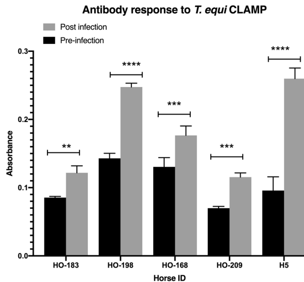
Figure 4. CLAMP elicits antibody responses in horses during infection with T. equi . CLAMP-specific antibodies are significantly present in horses after infection with T. equi (post-infection). ** p=0.0014 , *** p=0.0002 , **** p<0.0001 .
