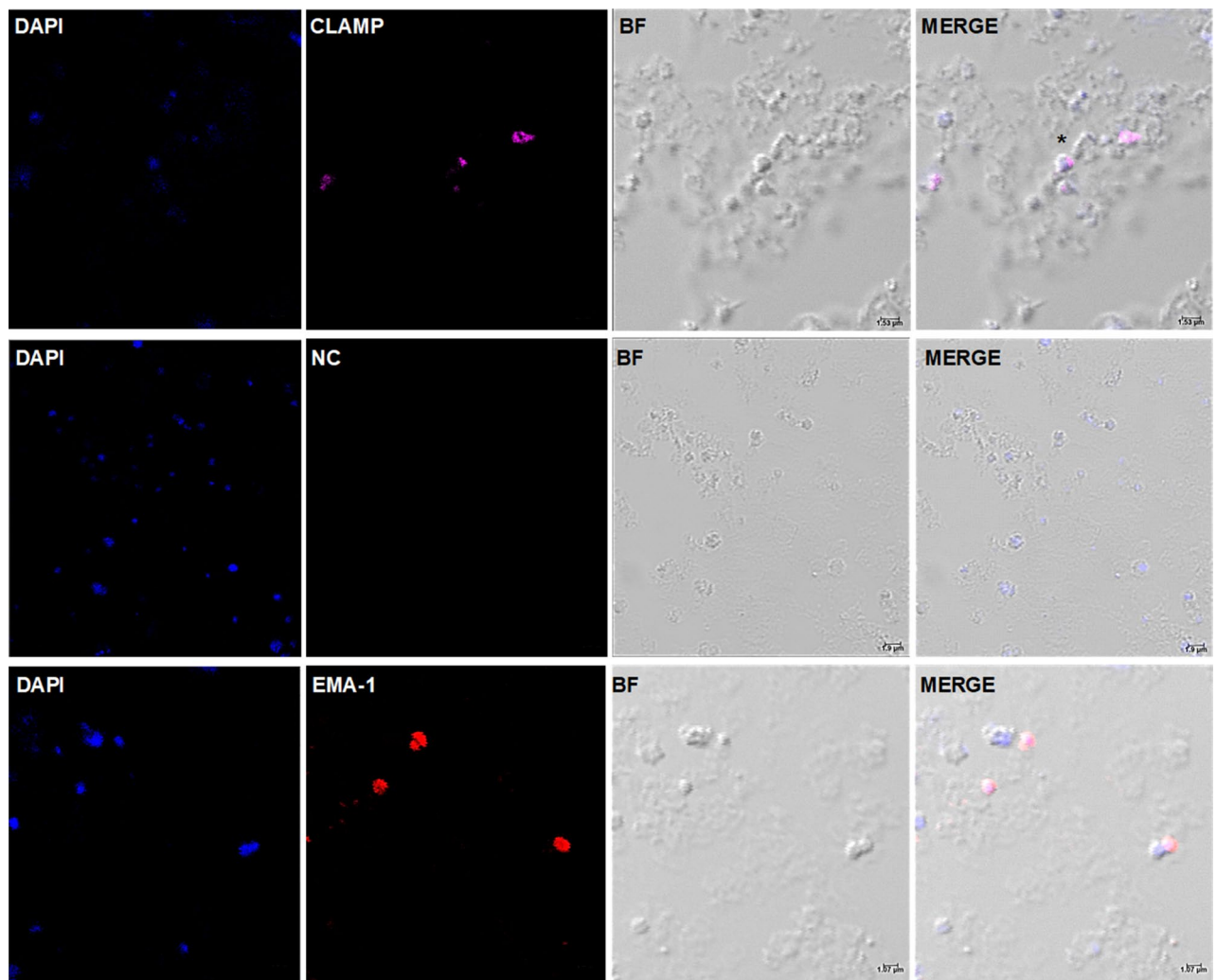
Figure 2. CLAMP is expressed on the surface of T. equi merozoites. Confocal microscopy images showing expression of CLAMP by extracellular T. equi merozoites. The first row shows expression of CLAMP on the surface of an extracellular merozoite (indicated by an asterisk (*)). The nuclei are stained in blue with DAPI, and CLAMP is stained in magenta. The second row represents merozoites incubated with the pre-immunization serum (negative control (NC)) and shows lack of protein staining indicating that the staining in the first row was CLAMP-specific. The third row shows expression of EMA-1 (positive control (PC)) by merozoites. In all cases, BF refers to brightfield panels.
