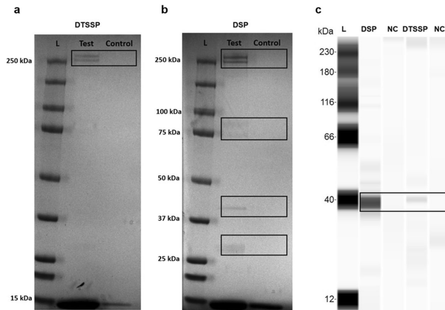
Figure 6. T. equi CLAMP interacts with equine erythrocyte proteins. (a,b) show SDS-PAGE gels of proteins (within black boundaries) isolated from the erythrocyte surface (test) and within the cell membrane and cell (test) after crosslinking to CLAMP with DTSSP and DSP, respectively. (c) Represents an immunoblot showing the presence of CLAMP at ~39 kDa. In all cases agarose resin eluates were used as negative controls (control/NC). The ~15 kDa band on the SDS-PAGE gels indicate non-specific binding of the equine \alpha - and \beta -hemoglobin subunits to the Thermo Scientific AminoLink (test) and agarose (control) coupling resins.
