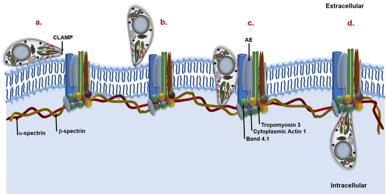
Figure 7. Hypothetical model showing the role of T. equi CLAMP in invasion of equine erythrocytes and its interactions with membrane skeleton proteins. (a) T. equi attaches to the equine erythrocyte surface, and (b) reorientates itself such that the apical end is in direct association with the cell membrane. (c) The parasite uses CLAMP (that is possibly translocated from the micronemes to the cell surface) to attach to the \alpha - and \beta -spectrin proteins during the initial stages of invasion. (d) Once inside the cell, T. equi CLAMP maintains its interactions with the spectrin proteins while also interacting with band 4.1, tropomyosin 3, cytoplasmic actin 1 and anion-exchange protein (AE).
