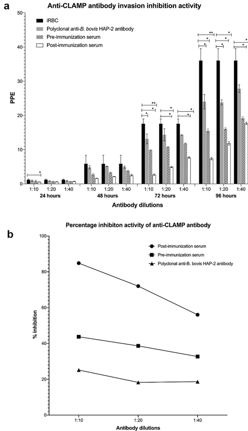
Figure 5. Polyclonal anti-CLAMP antibody significantly inhibits invasion of equine erythrocytes by T. equi . (a) In vitro neutralization assay data showing invasion inhibition activity of the CLAMP-specific antibody (post-immunization serum), pre-immunization serum and polyclonal anti- B. bovis HAP-2 antibody at different dilutions over time. T. equi infected erythrocytes cultured in the presence of CLAMP-specific antibodies were significantly less parasitized (PPE) compared to parasites cultured in the presence of pre-immunization serum and the polyclonal anti- B. bovis HAP-2 antibody. Control represents T. equi infected red blood cells (iRBC) cultured in the absence of both pre- and post-immunization sera. * p < 0.05 , ** p < 0.0090 . (b) Anti-CLAMP antibodies inhibit a significant percentage of parasites from invading erythrocytes at 72 h post-infection. Percentage inhibition was calculated as the difference between percentage inhibition in the presence of polyclonal anti-CLAMP antibodies (post-immunization serum) and percentage inhibition in the presence of pre-immunization serum. In this regard, anti-CLAMP antibodies in the post-immunization serum inhibited parasite invasion by 41%, 33.4% and 23.3% at 1:10, 1:20 and 1:40 dilutions, respectively. Factors present in the B. bovis HAP-2 post immunization serum (polyclonal anti- B. bovis HAP-2 antibody) also minimally inhibited invasion.
