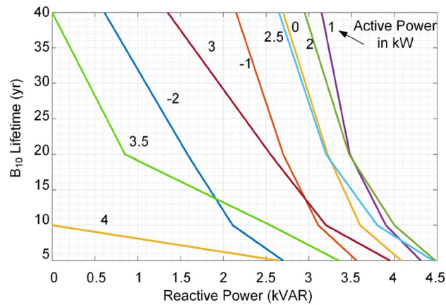
Figure 10. B_{10} lifetime curves versus reactive power and active power.
