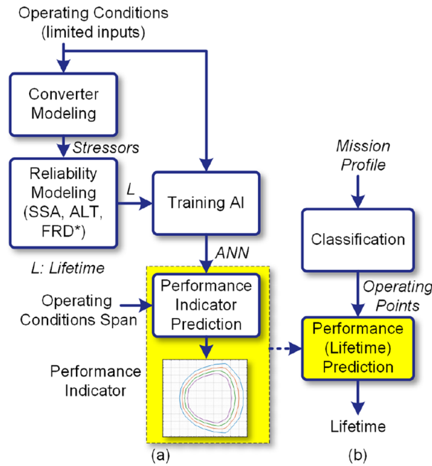
Figure 2. Proposed AI-based long-term performance prediction in converters, (a) performance indicator prediction, (b) application of performance index in lifetime estimation. *SSA stress-strength analysis, ALT accelerated life test, FRD field returned data.
