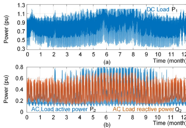
Figure 17. Annual load profiles; (a) dc load power, and (b) ac load active and reactive power.
