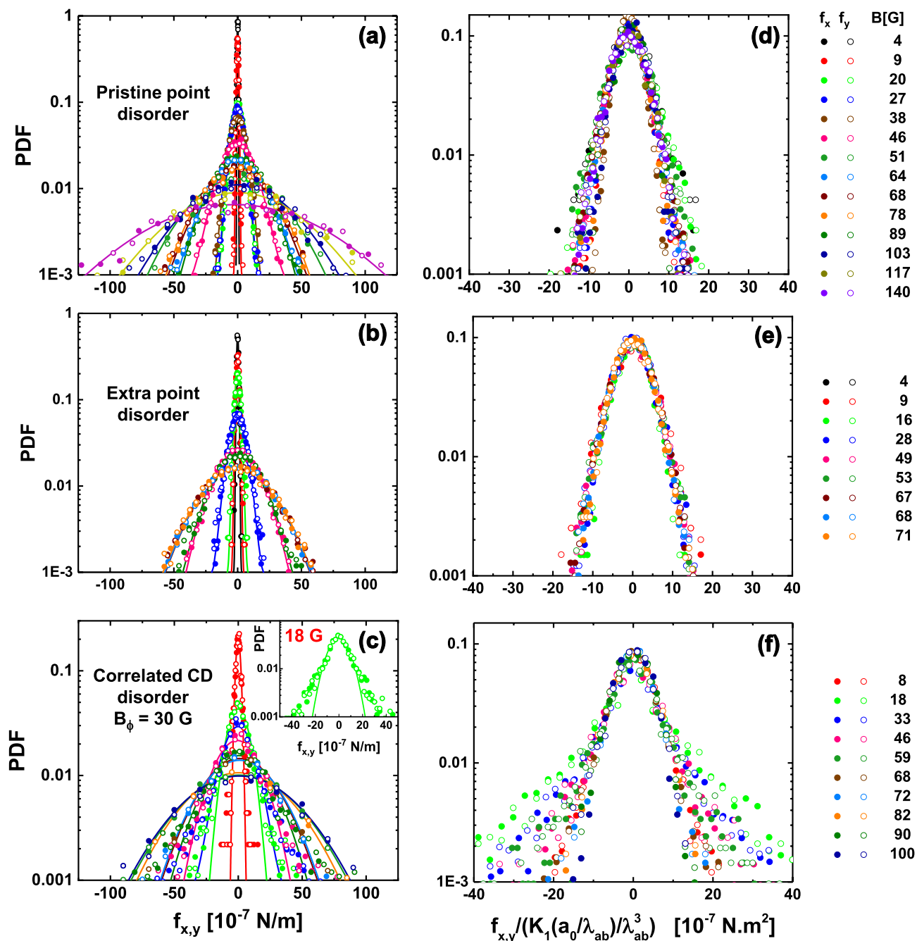
Figure 4. Probability density functions (PDFs) of the particle-particle interaction force components f_x (full points) and f_y (open points) for vortex structures nucleated at various applied fields in \text{Bi}_2\text{Sr}_2\text{CaCu}_2\text{O}_{8+\delta} samples with point (a) pristine, (b) electron irradiated, and (c) correlated CD disorder with B_\phi = 30 G. Data are presented in log-linear scale. Full lines are fits to the data with a Gaussian function \propto (1/\sigma_G) \cdot \exp(-x^2/2\sigma_G^2) in the whole force range. This function describe reasonably well the PDFs in the case of point disorder, but in the case of correlated disorder fail to follow the experimentally-observed tails that decay slowly with f_{x,y} than a Gaussian function. The inset in (c) shows the example of the 18 G data where it is evident that the Gaussian function (full green line) underestimates the experimental data in the large-force range. The right panels (d–f) show the PDFs of the left panels plot in log-linear scale with the x-axis normalized by the factor K_1(a_0/\lambda_{ab})/\lambda^3 and then normalized to have an area under the curve equal to one. In this representation, for point disorder the PDFs scale in a single evolution whereas for dilute correlated disorder the curves do not overlap in the large-force range.
