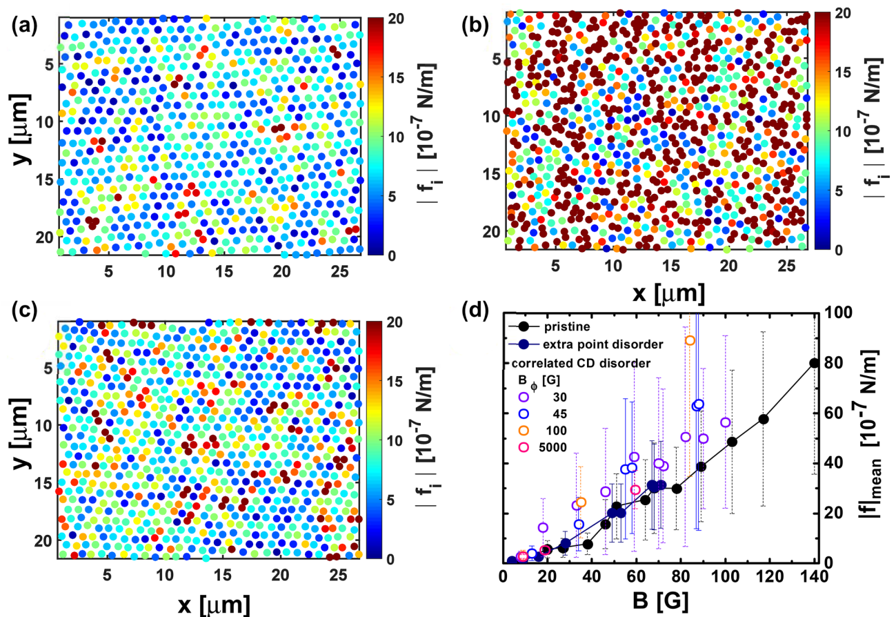
Figure 3. Colour-coded maps of the modulus of the particle-particle interaction force |f_i| for 30 G vortex structures nucleated in \text{Bi}_2\text{Sr}_2\text{CaCu}_2\text{O}_{8+\delta} samples with point ((a) pristine, (c) electron-irradiated) and correlated CD disorder ((b) heavy-ion irradiated with B_\phi = 30 G). (d) Density (field)-dependence of the mean value of |f_i| , |f|_{\text{mean}} , obtained from large field-of-view maps with 7000–15000 vortices for all the studied structures. Bars accompanying the points are not error bars but the value of the standard deviation of the |f_i| distribution registered in such extended fields-of-view.
