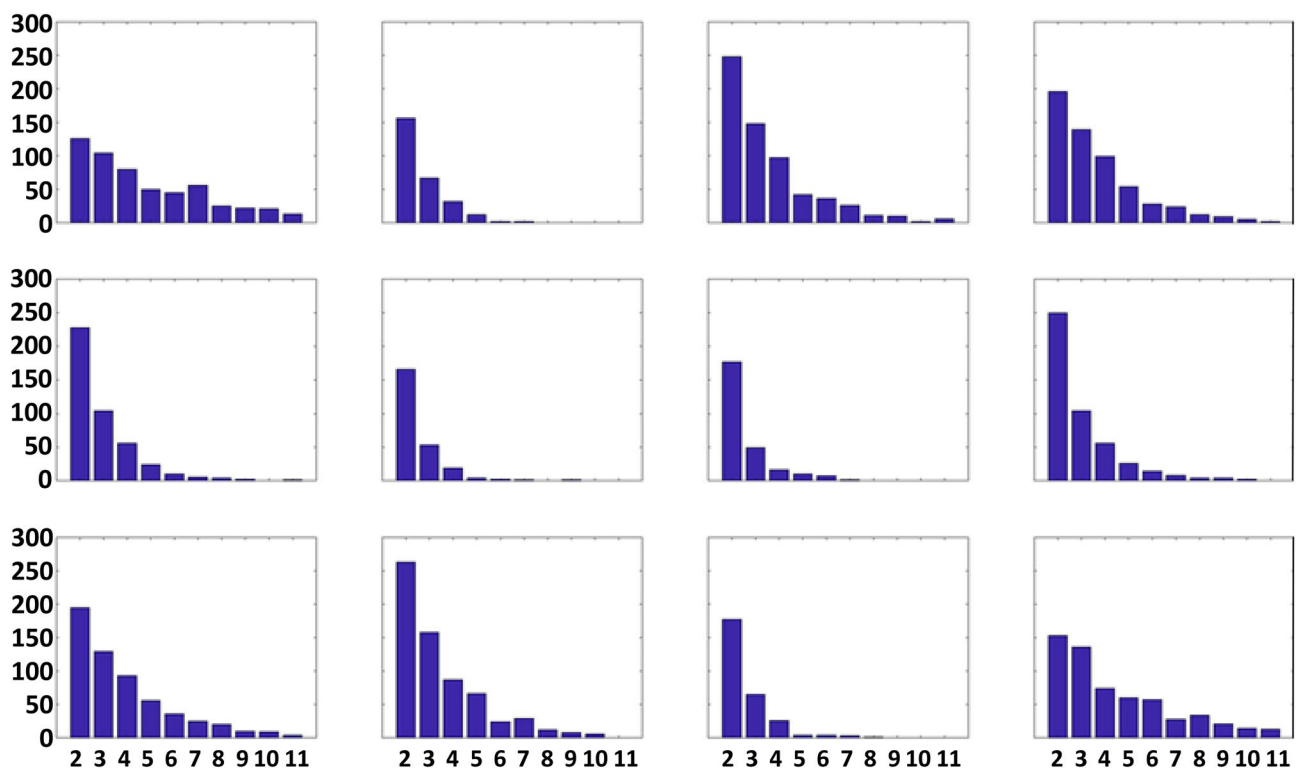
Figure 5. Distribution of LDEs of varying duration in each node. The horizontal axis is length of LDEs in days, and the vertical axis is total number of LDEs of each duration.
