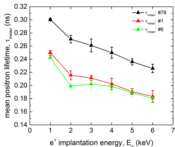
Figure 7. Mean lifetimes \tau_{mean} of positrons trapped at defects plotted as a function of the positron energy for three samples: cavity-cut outs #1 and #6 and sample 78.
