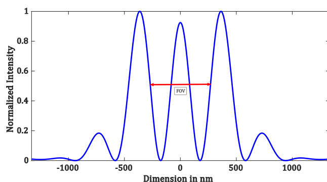
Figure 8. FOV measurement.
